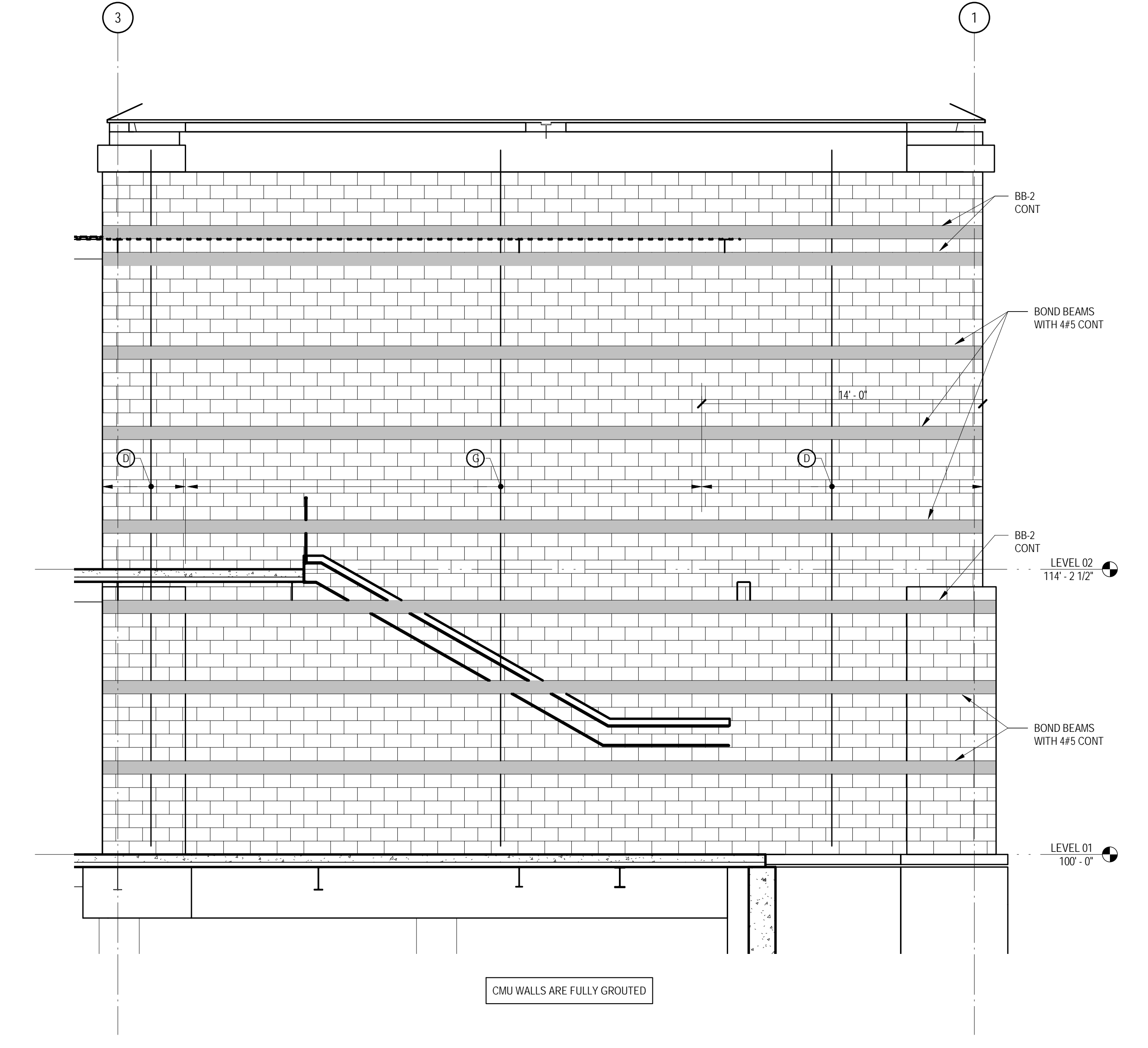
12 WALL ELEVATION AT GRID A 1/4" = 1'-0"
