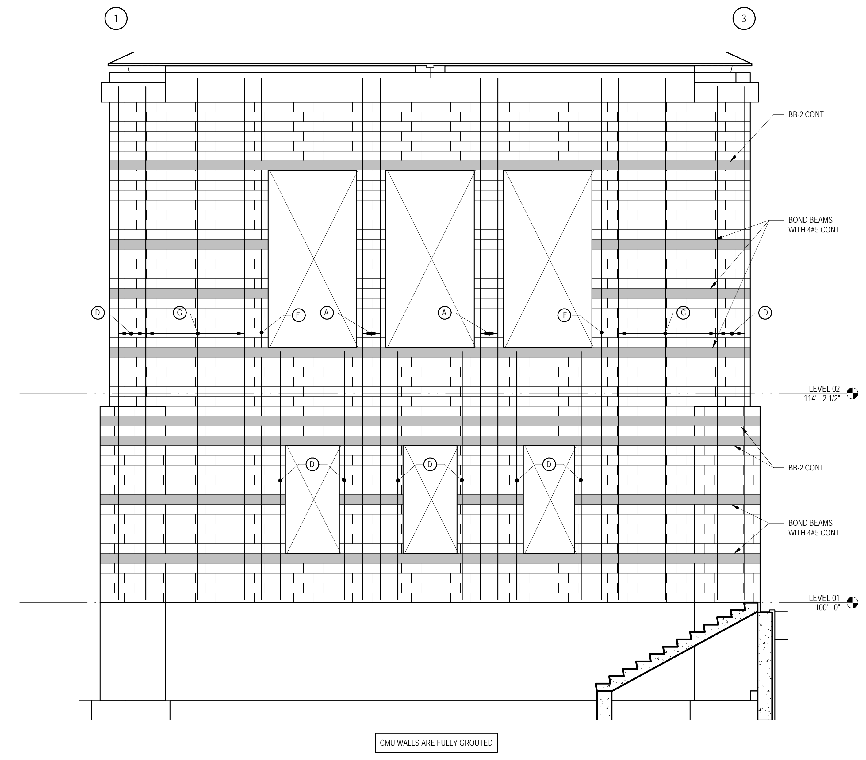
18 WALL ELEVATION AT GRID F 1/4" = 1'-0"
