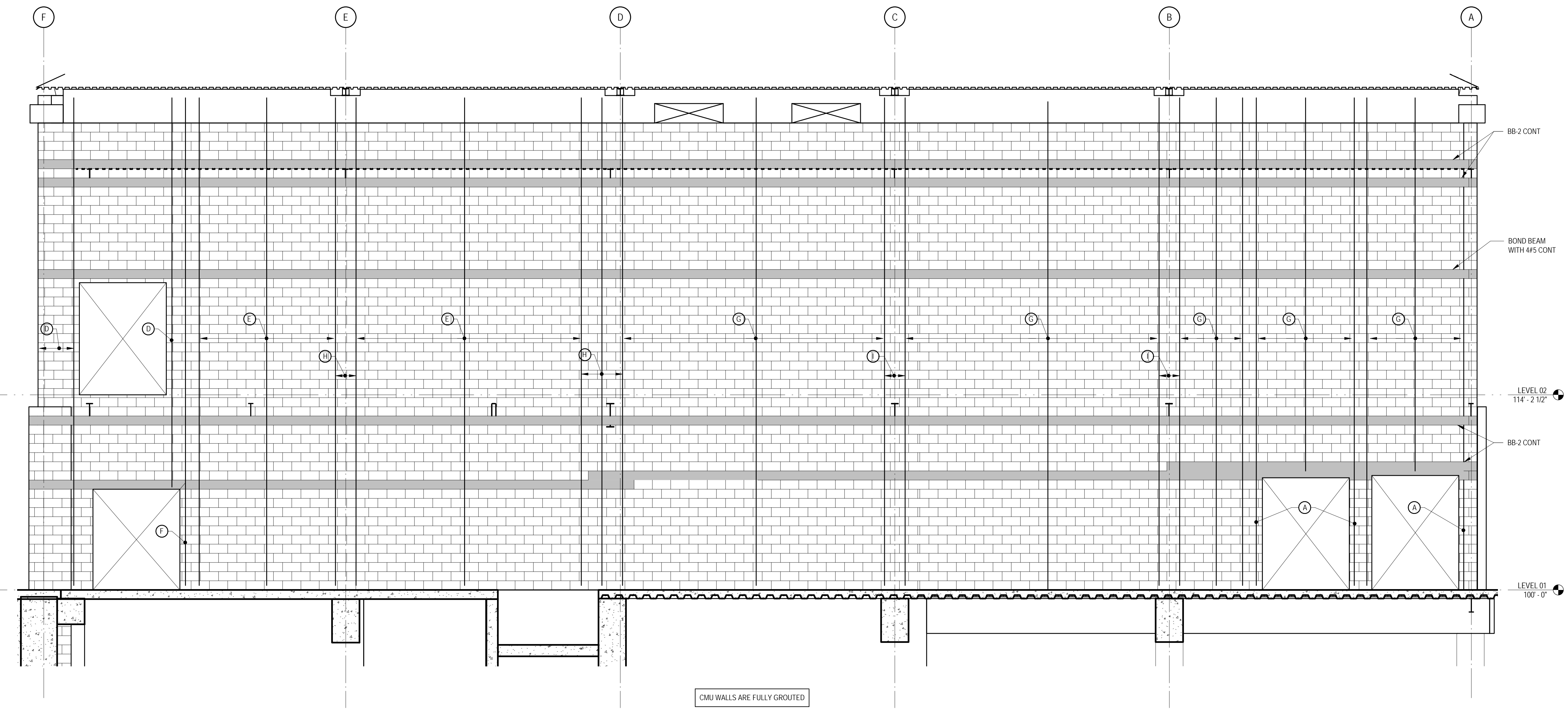
24 WALL ELEVATION AT GRID 3 1/4" = 1'-0"
