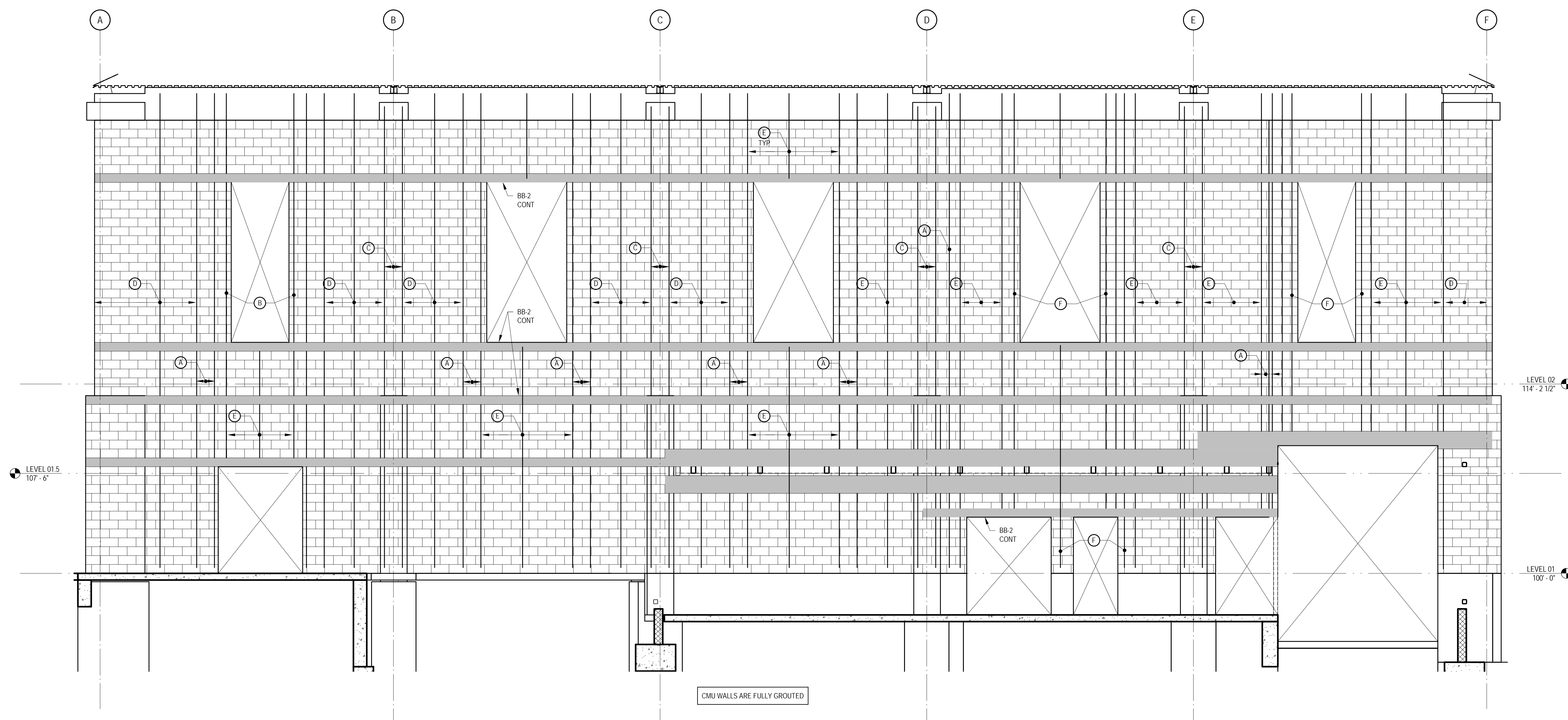
22 WALL ELEVATION AT GRID 1 1/4" = 1'-0"
