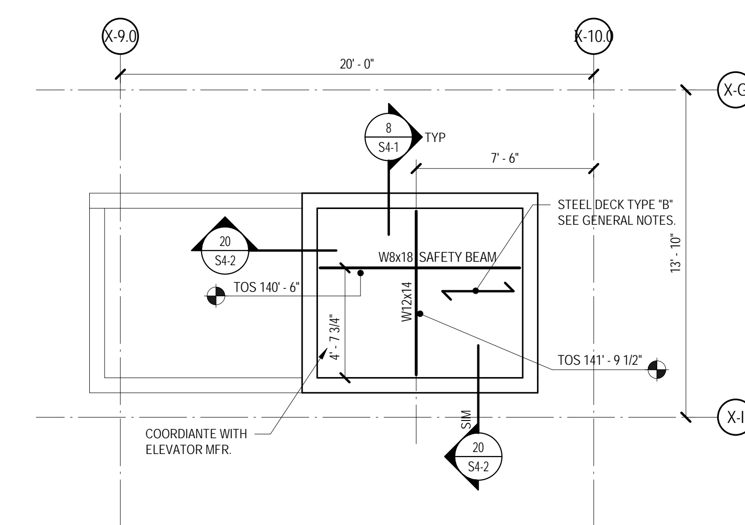
2 ELEVATOR SHAFT POP UP ROOF 1/4" = 1'-0"
