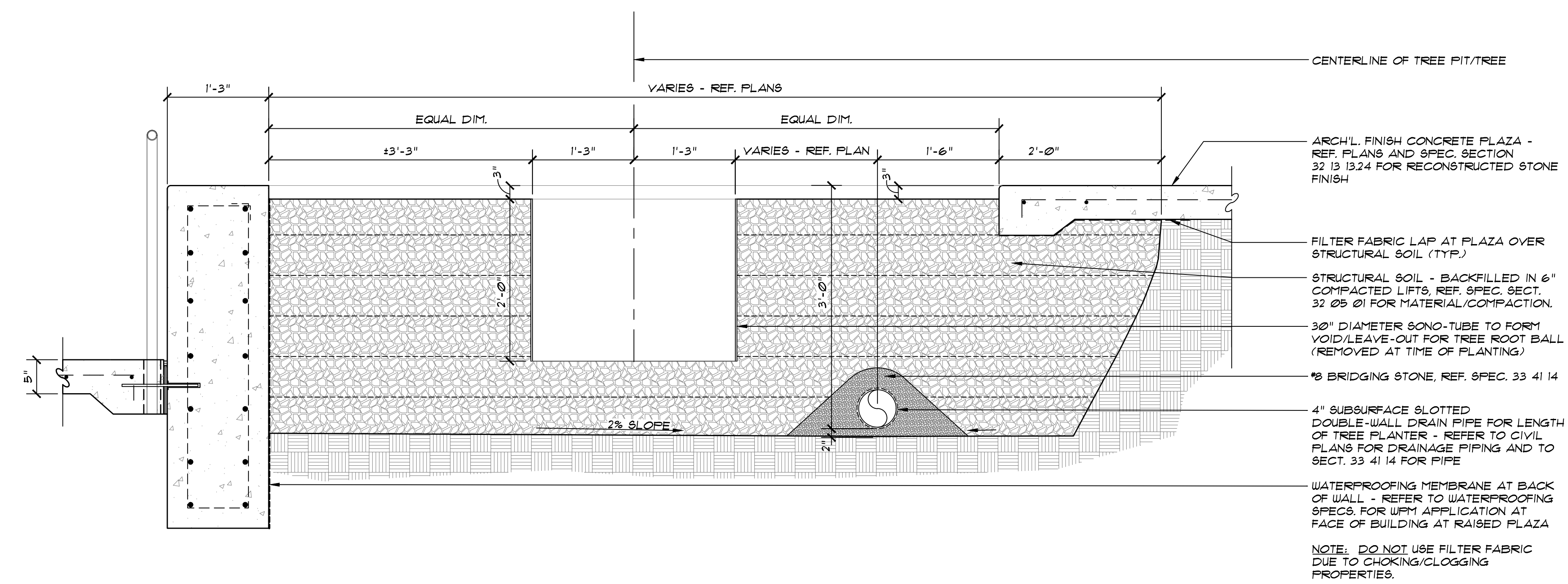
2 TREE PLANTER AT PLAZA - STRUCTURAL SOIL & SUBSURFACE DRAIN - SECTION 1" = 1'-0"
