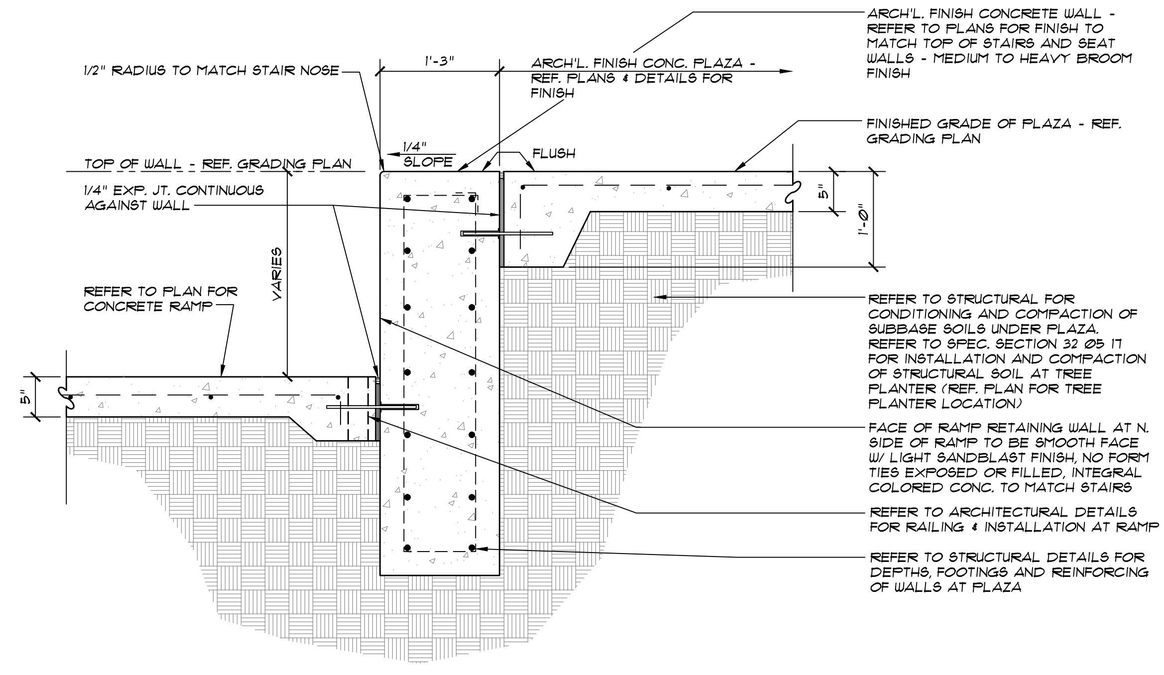
3 WALL DETAIL BETWEEN RAMP & UPPER PLAZA - SECTION 1" = 1'-0"
