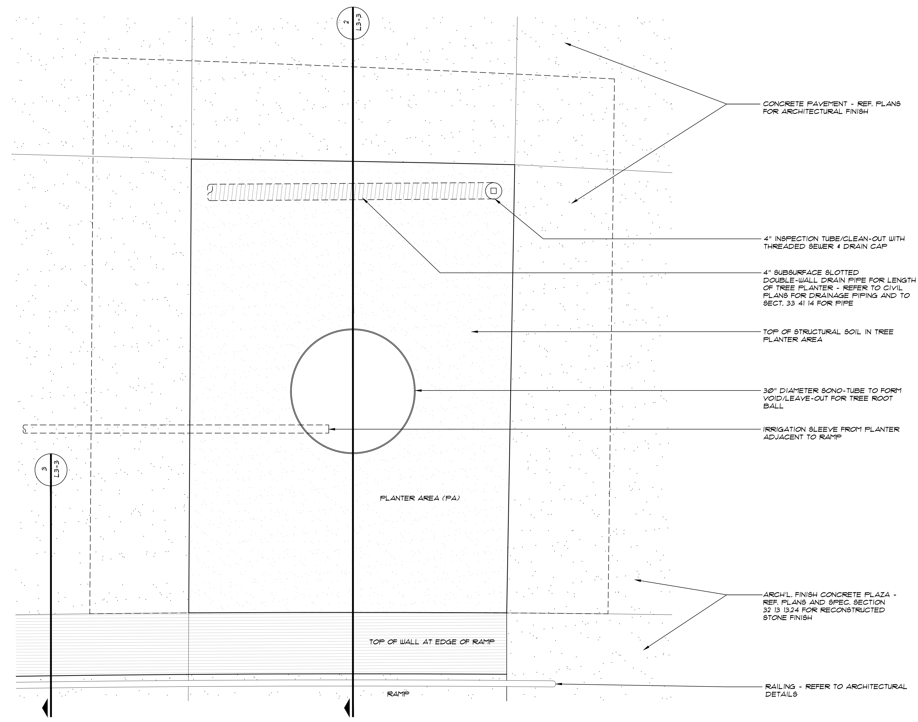
1 TREE PLANTER AT PLAZA - STRUCTURAL SOIL & SUBSURFACE DRAIN - PLAN 1" = 1'-0"
