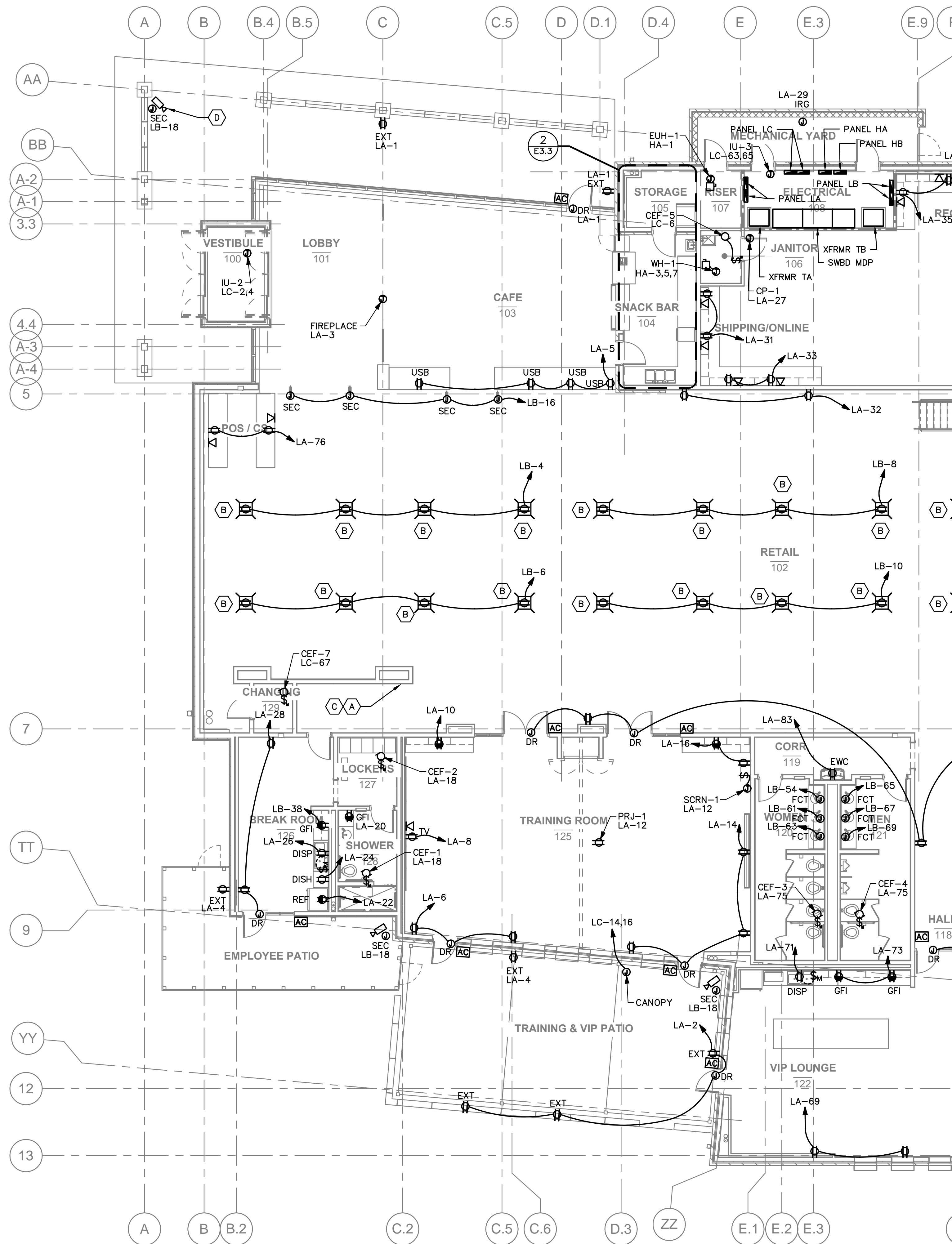
POWER FLOOR PLAN - LEVEL 1 - AREA A 1 SCALE: 1/8" = 1'-0" E3.1
