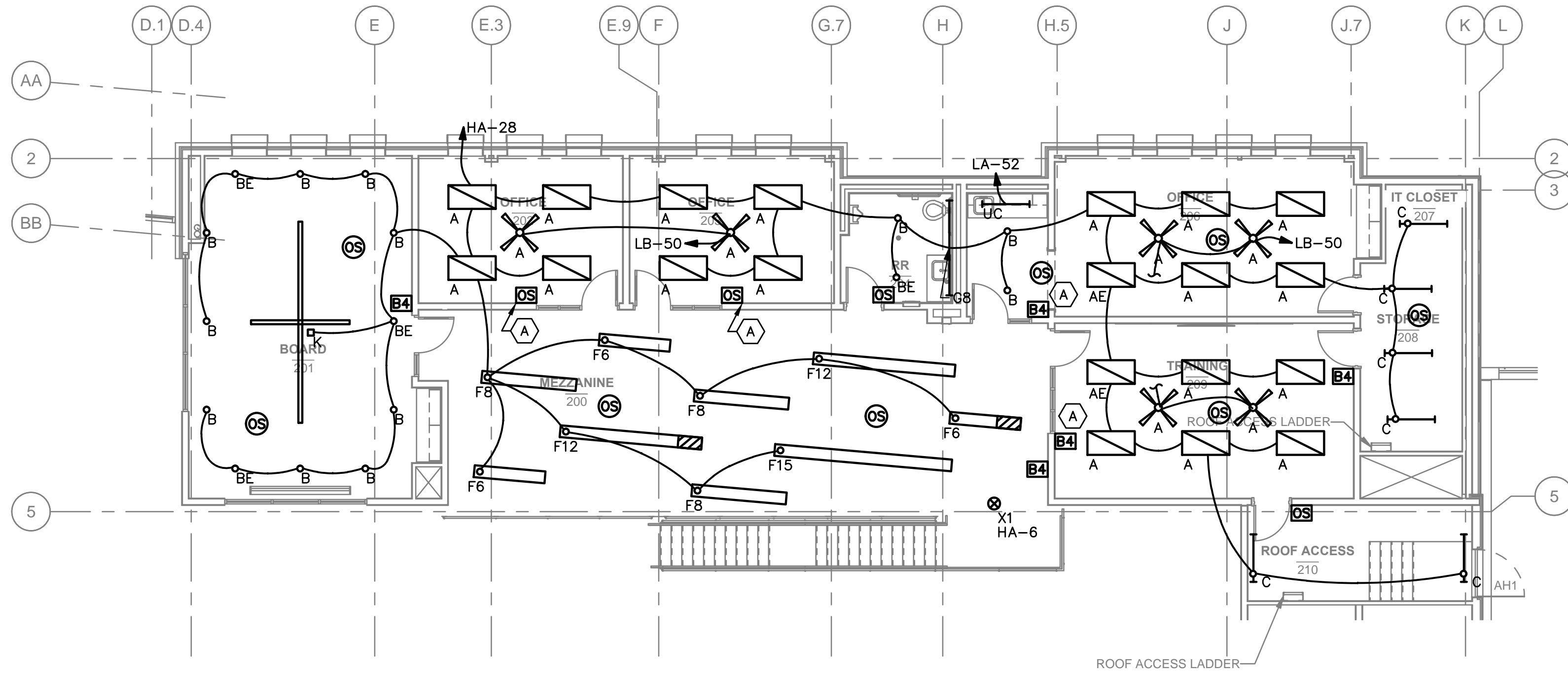
LIGHTING FLOOR PLAN - MEZZANINE 1 SCALE: 1/8" = 1'-0" E2.3
