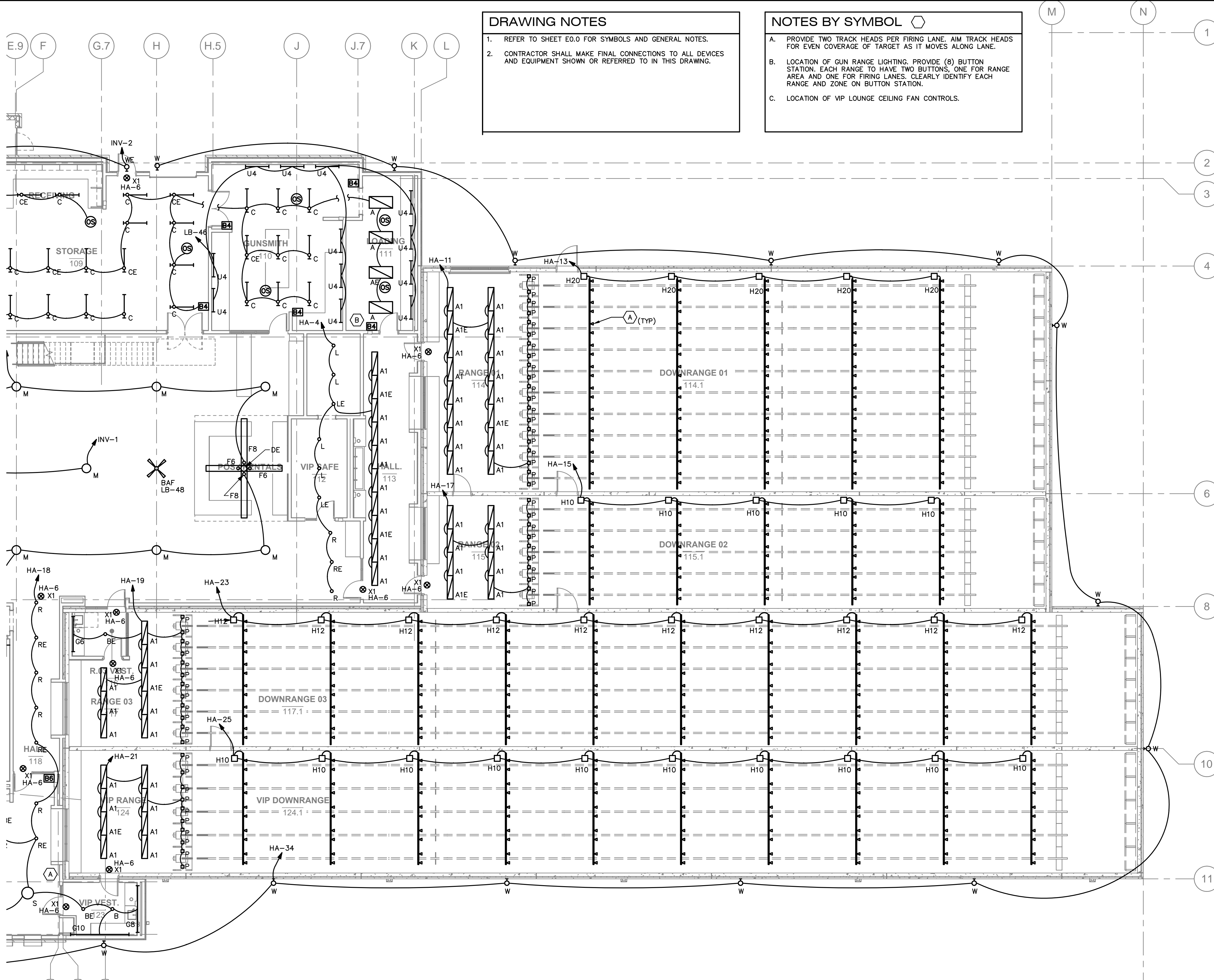
LIGHTING FLOOR PLAN - LEVEL 1 - AREA B 1 SCALE: 1/8" = 1'-0" E2.2
