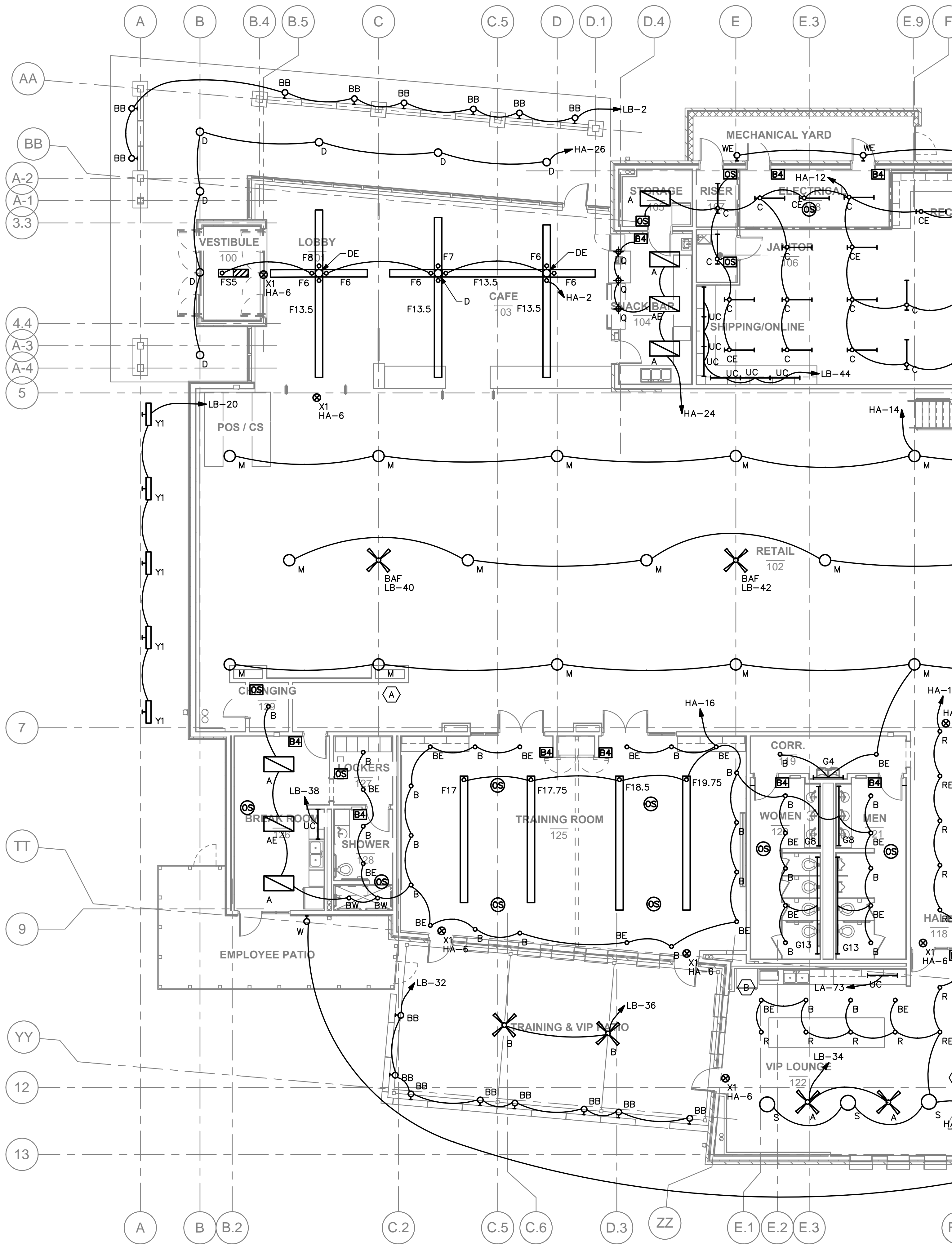
LIGHTING FLOOR PLAN - LEVEL 1 - AREA A SCALE: 1/8" = 1'-0" E2.1
