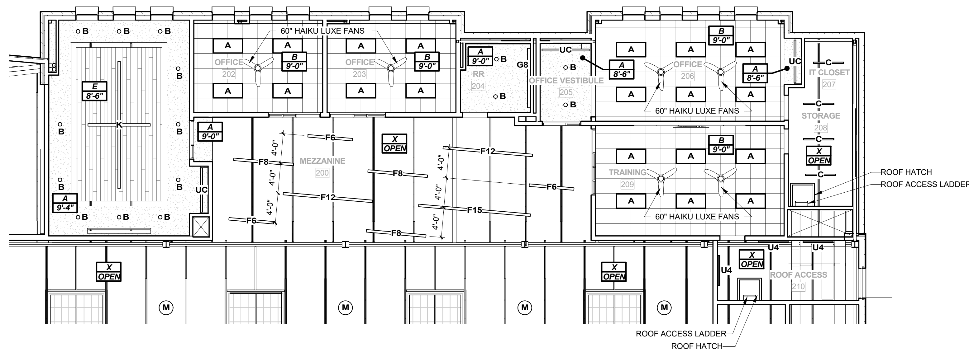
REFLECTED CEILING PLAN - LEVEL 1 - MEZZANINE | 1 SCALE: 1/8" = 1'-0" | A2.23
