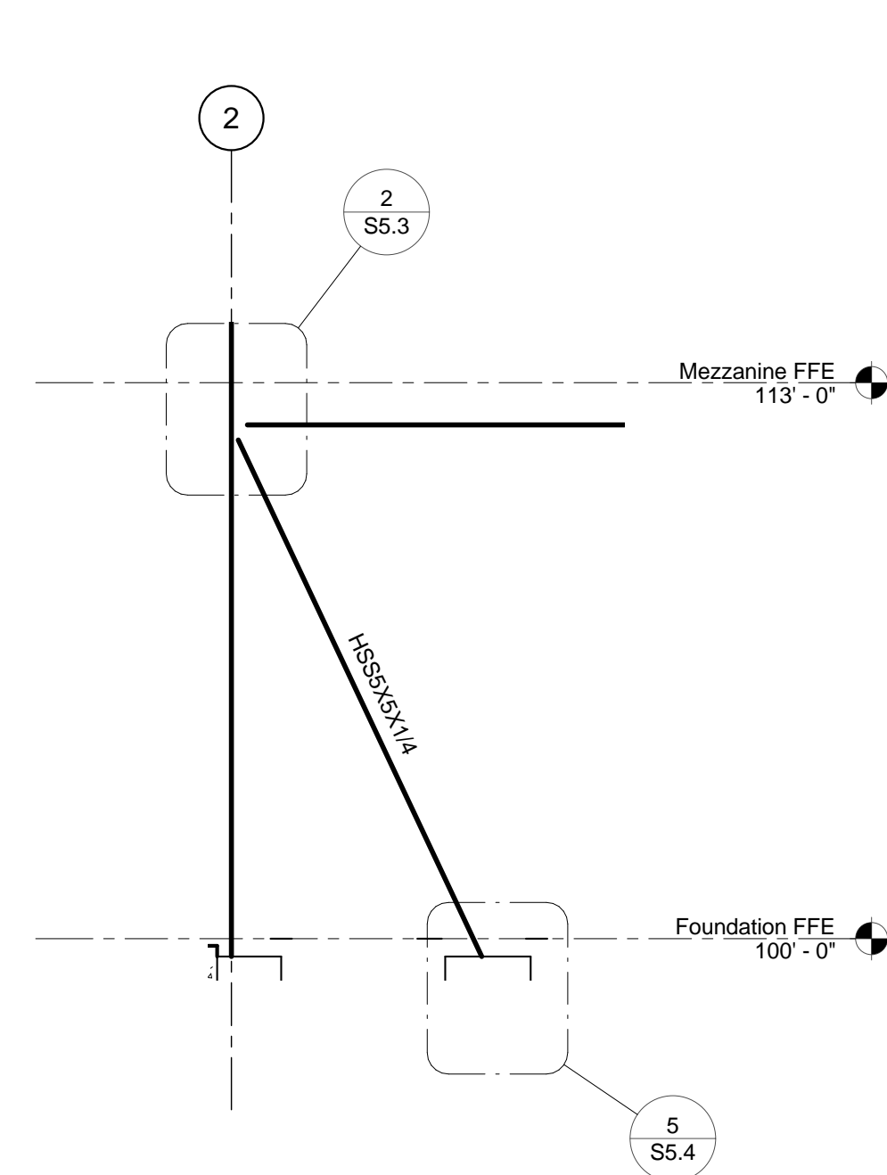
3 BRACE ELEVATION
