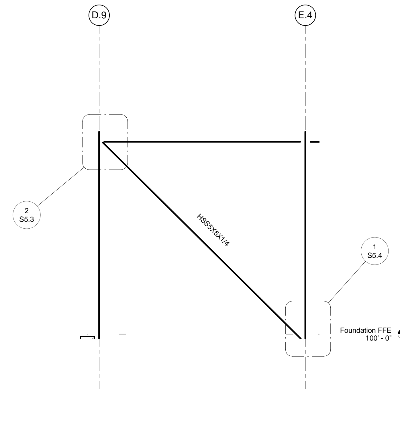
2 BRACE ELEVATION
