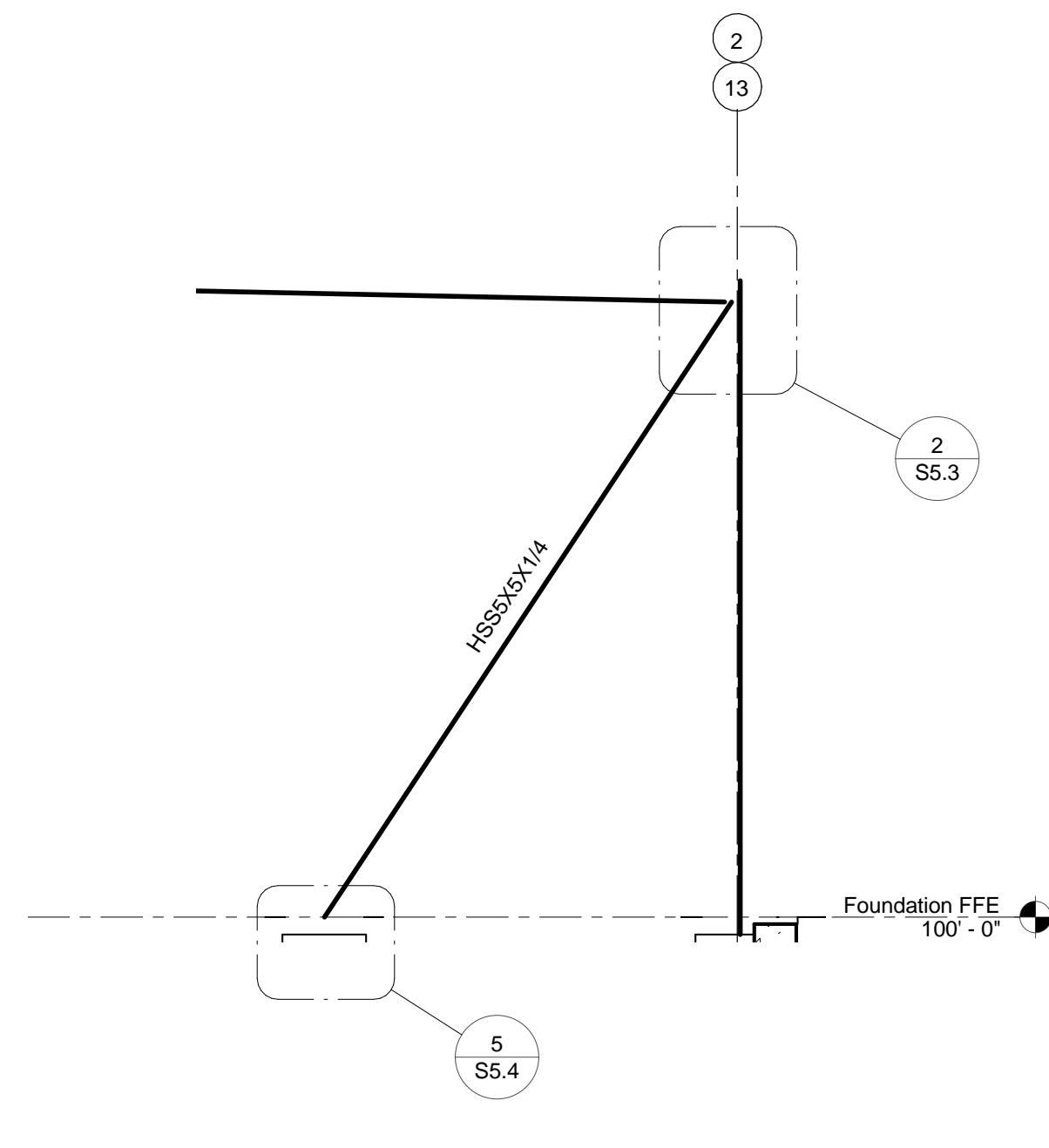
4 BRACE ELEVATION
