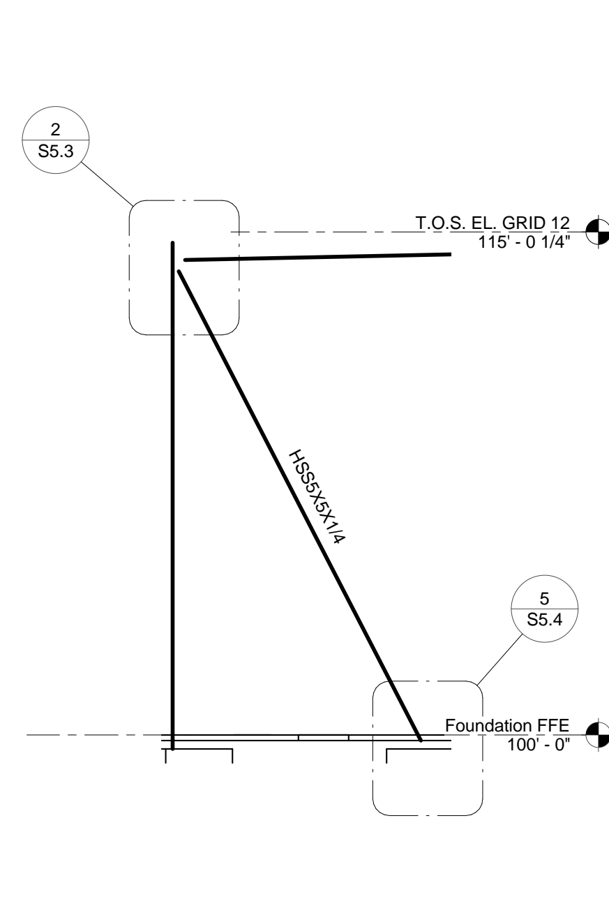
5 BRACE ELEVATION
