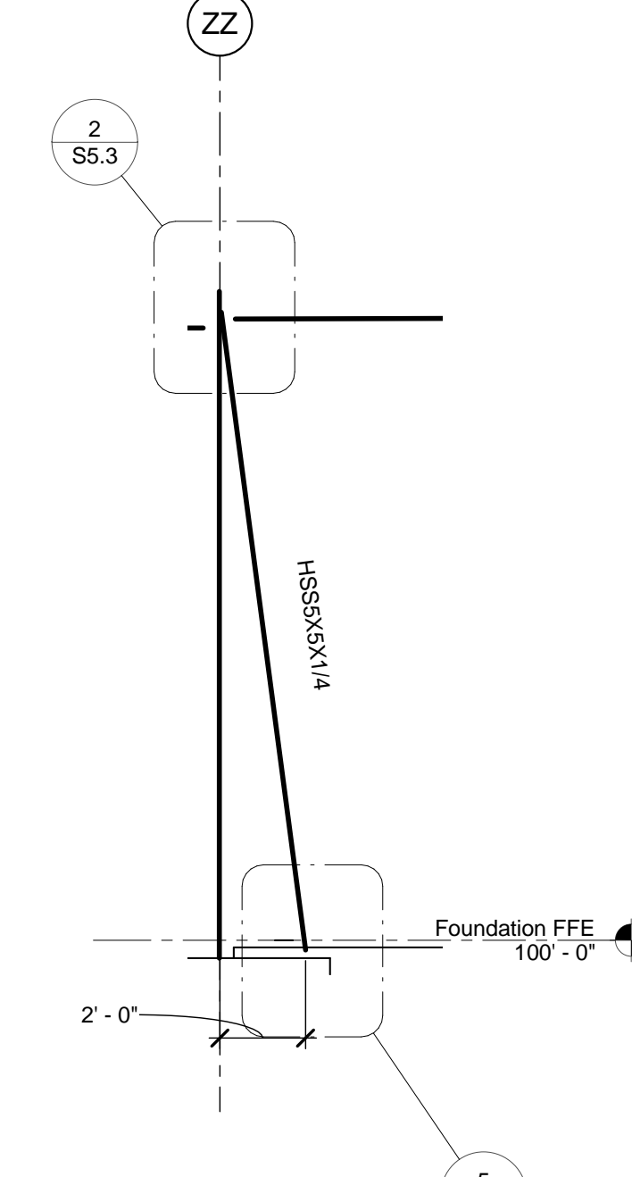
6 BRACE ELEVATION
