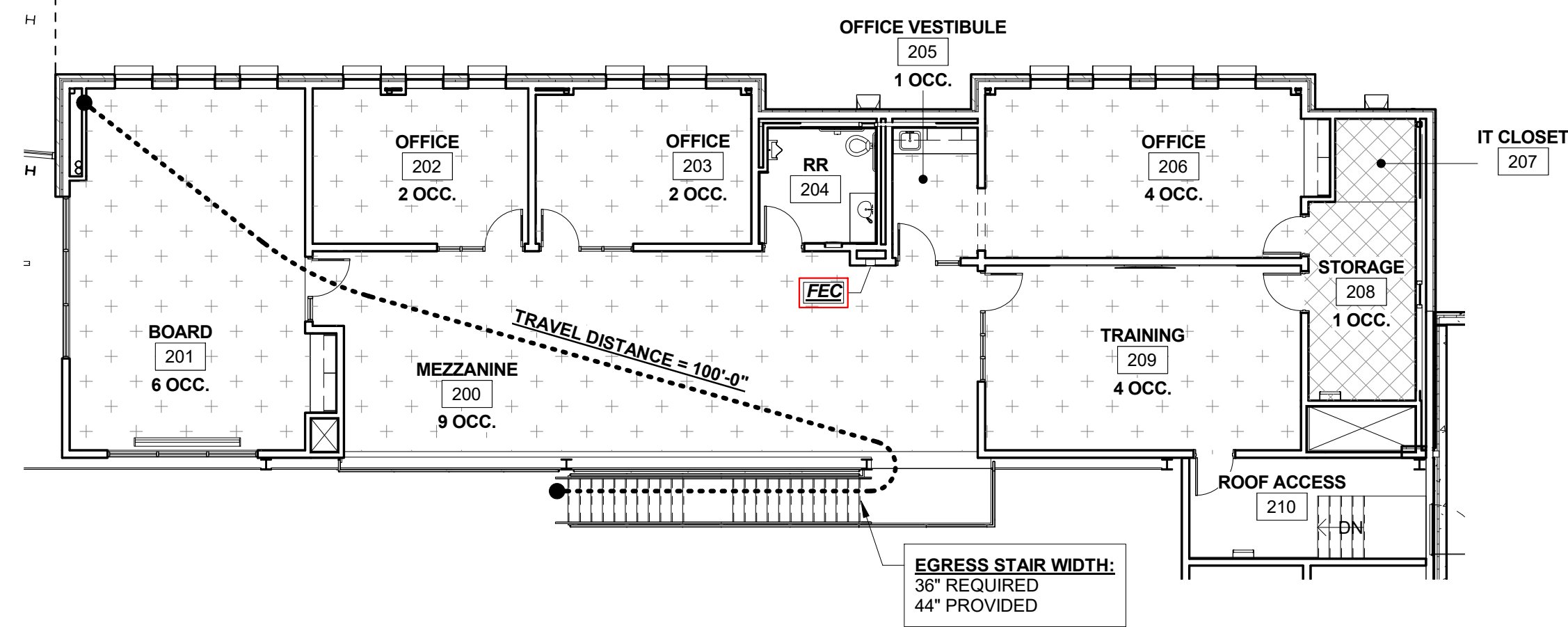
LIFE SAFETY PLAN - MEZZANINE | 2
