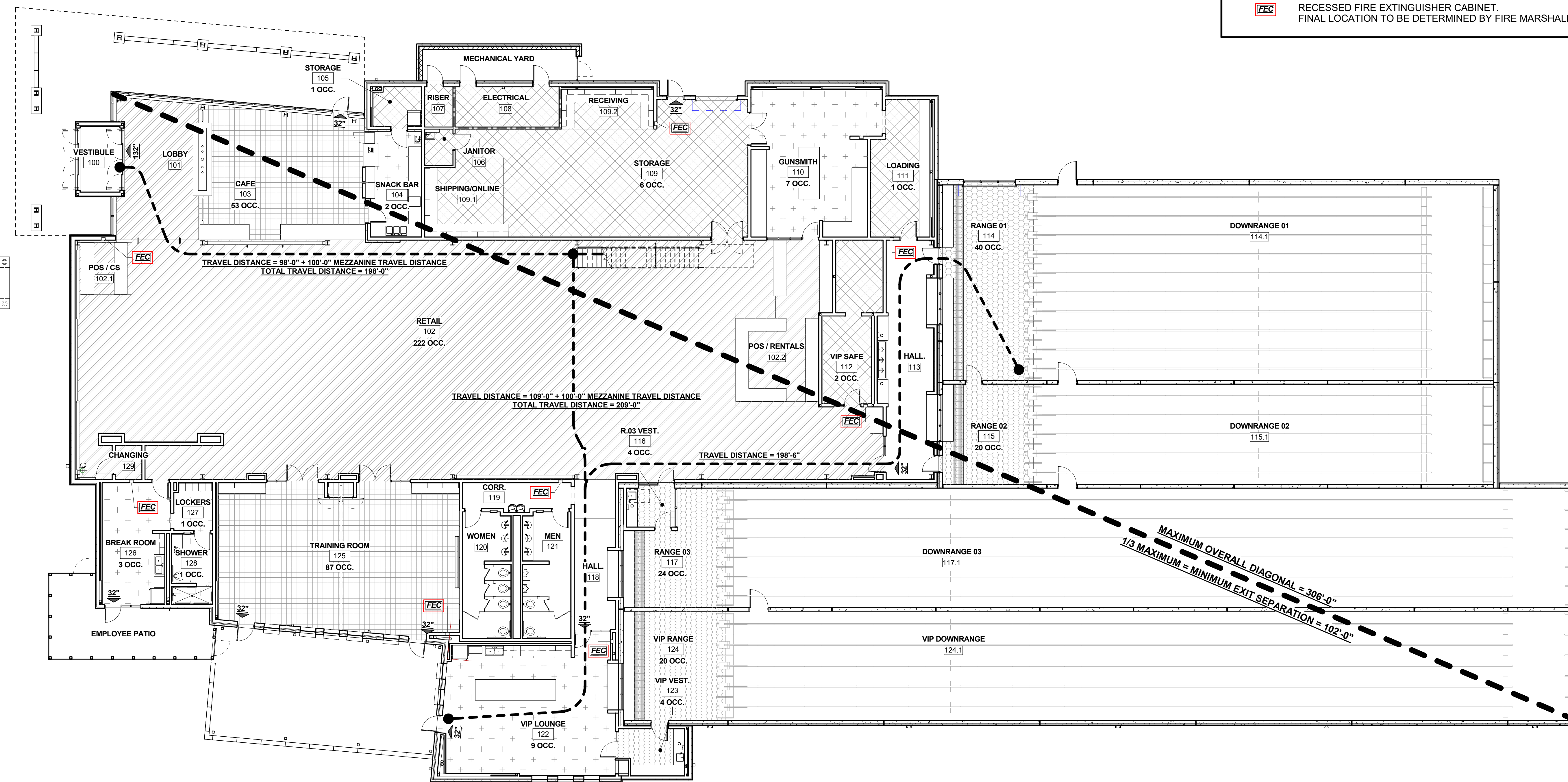
LIFE SAFETY PLAN - LEVEL 1 | 1
