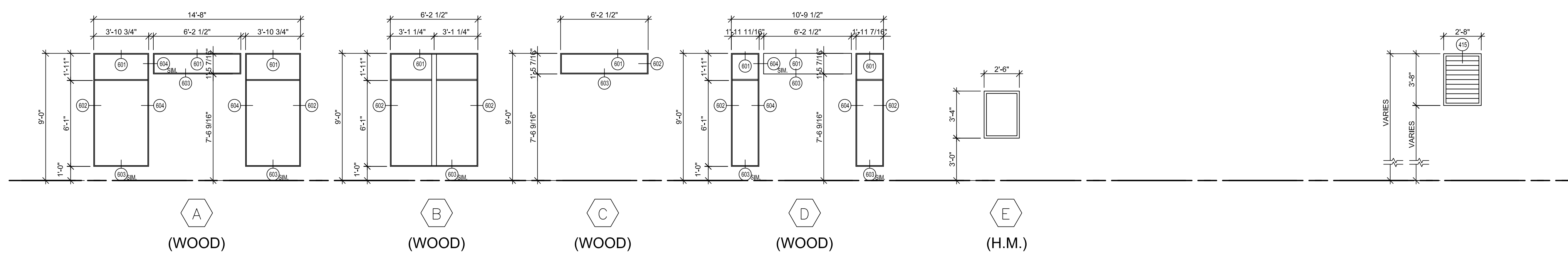
BORROWED LIGHT ELEVATIONS GLAZING: 1/4" CLEAR TEMPERED
