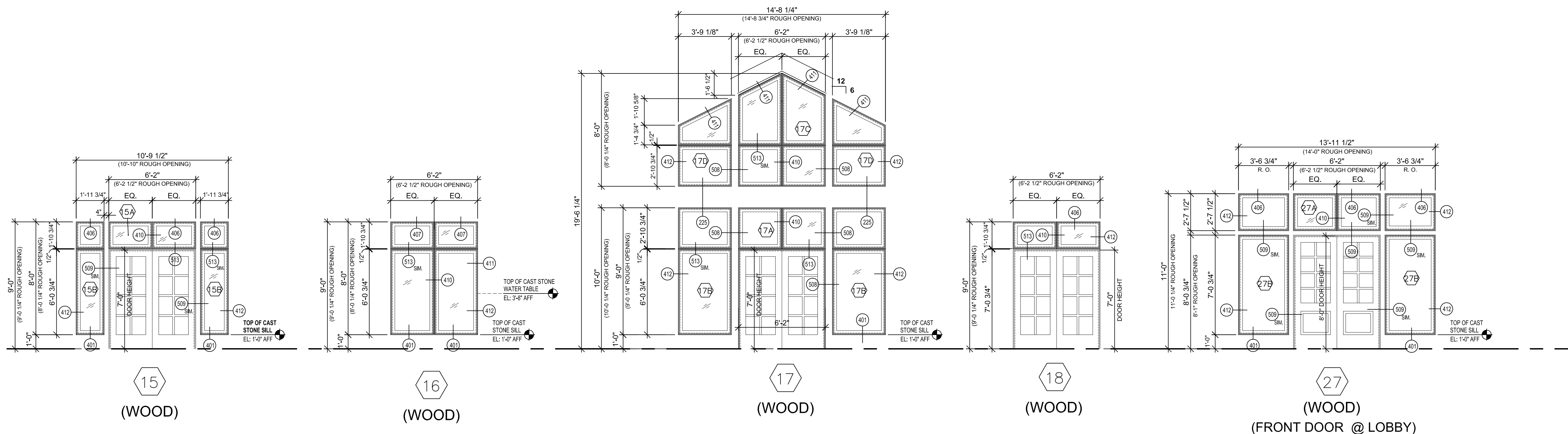
EXTERIOR WINDOW ELEVATIONS - WOOD GLAZING: 1" INSULATED
