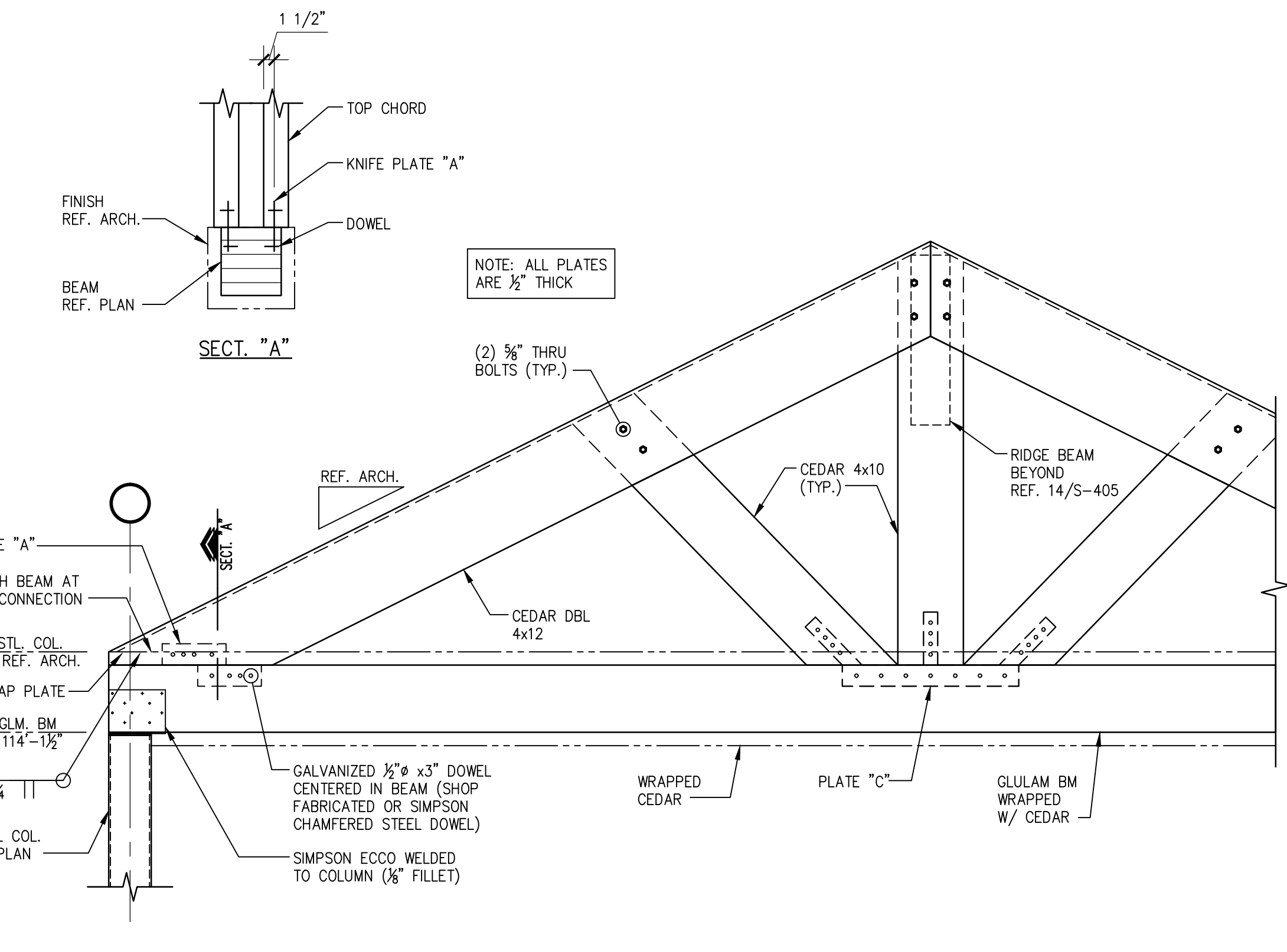
11 PARTIAL TRUSS ELEVATION SCALE: 3/4"=1'-0"
