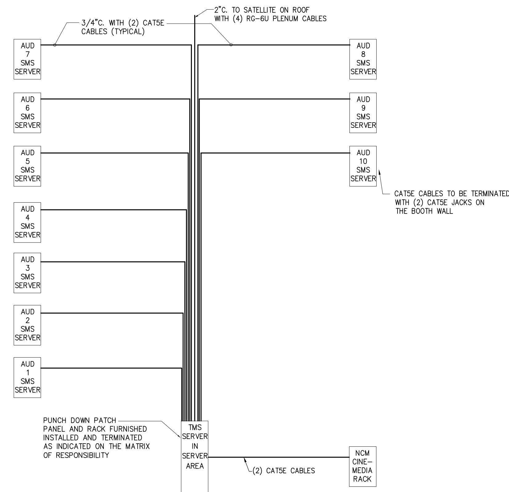
05 DIGITAL CINEMA RISER DIAGRAM SCALE: NO SCALE
