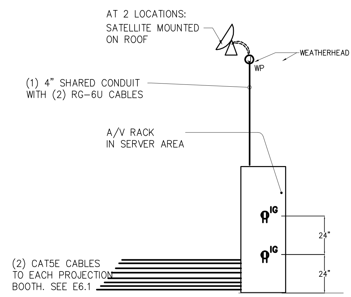
03 DIGITAL ADVERTISING A/V RISER DIAGRAM SCALE: NONE
