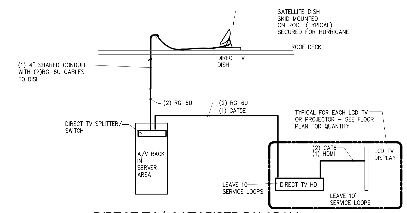
07 DIRECT TV / CATV RISER DIAGRAM SCALE: NO SCALE
