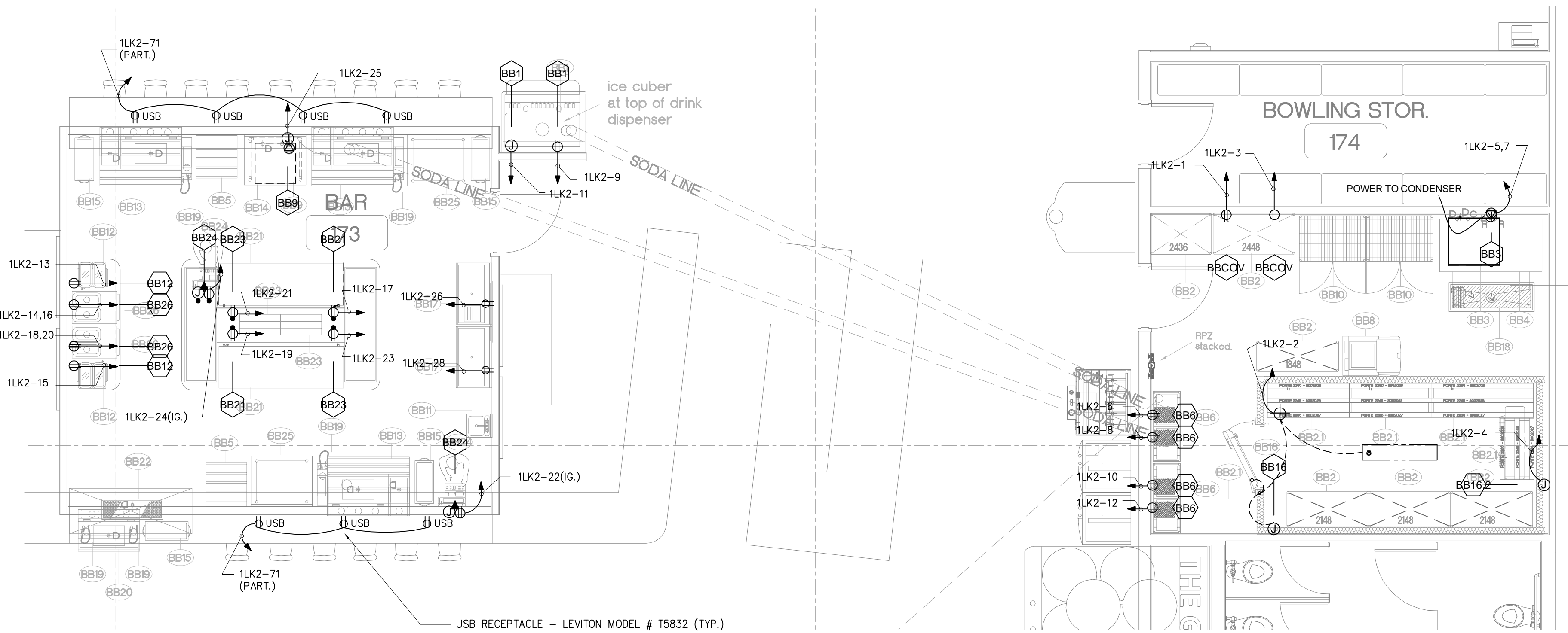
02 ENLARGED BAR PLAN - POWER SCALE: 1/4"=1'-0"
