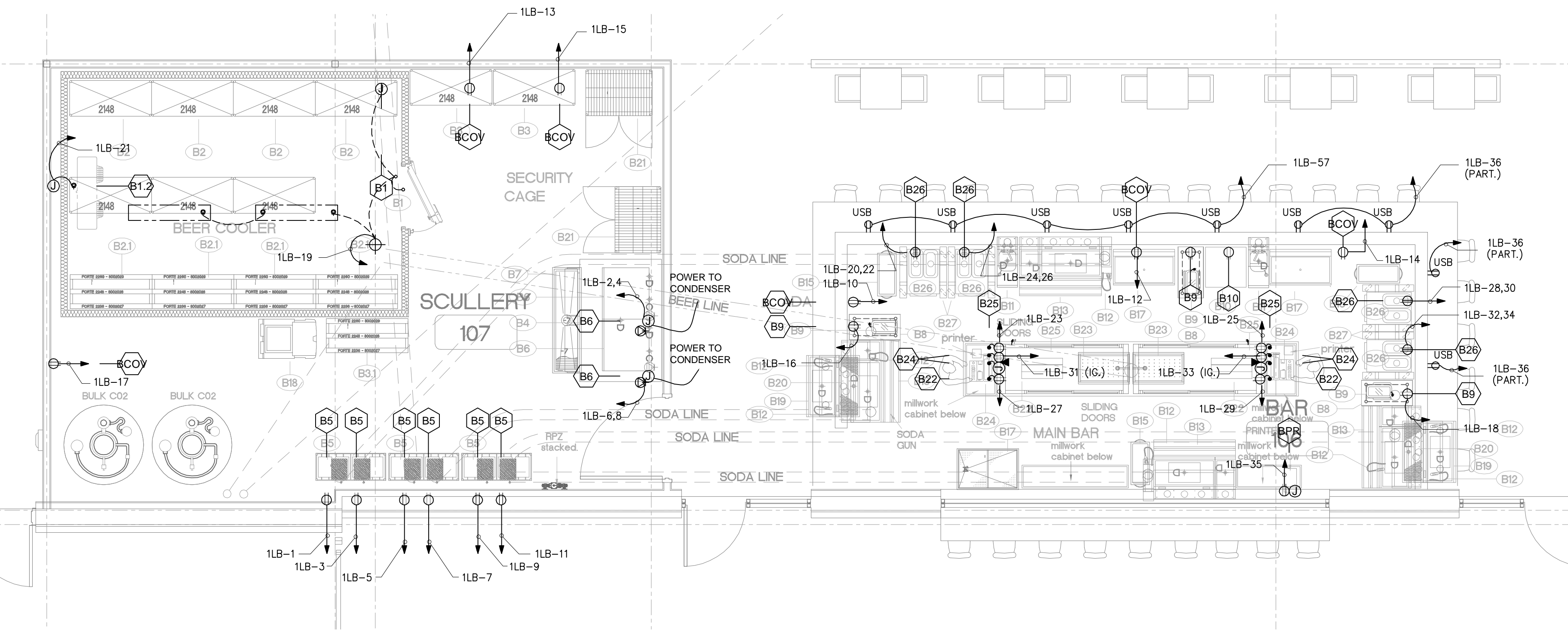
01 ENLARGED BAR PLAN - POWER SCALE: 1/4"=1'-0"
