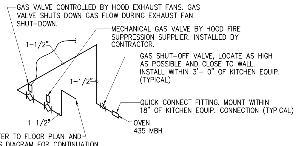
09 OVEN GAS RISER Scale: NOT TO SCALE
