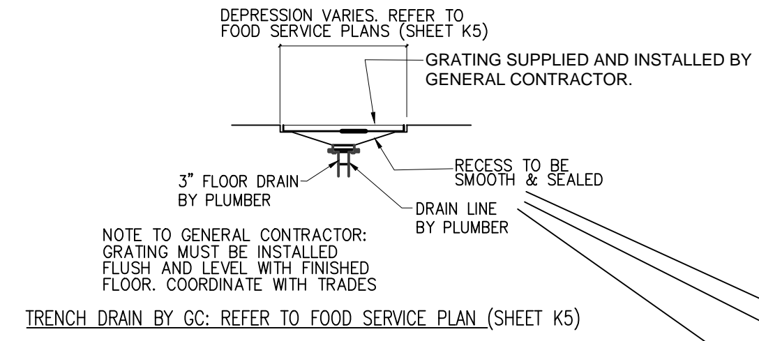
04 3-COMP. SINK DETAIL Scale: NOT TO SCALE
