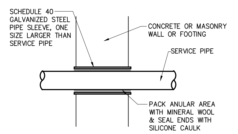
07 PIPE PENETRATIONS Scale: NOT TO SCALE
