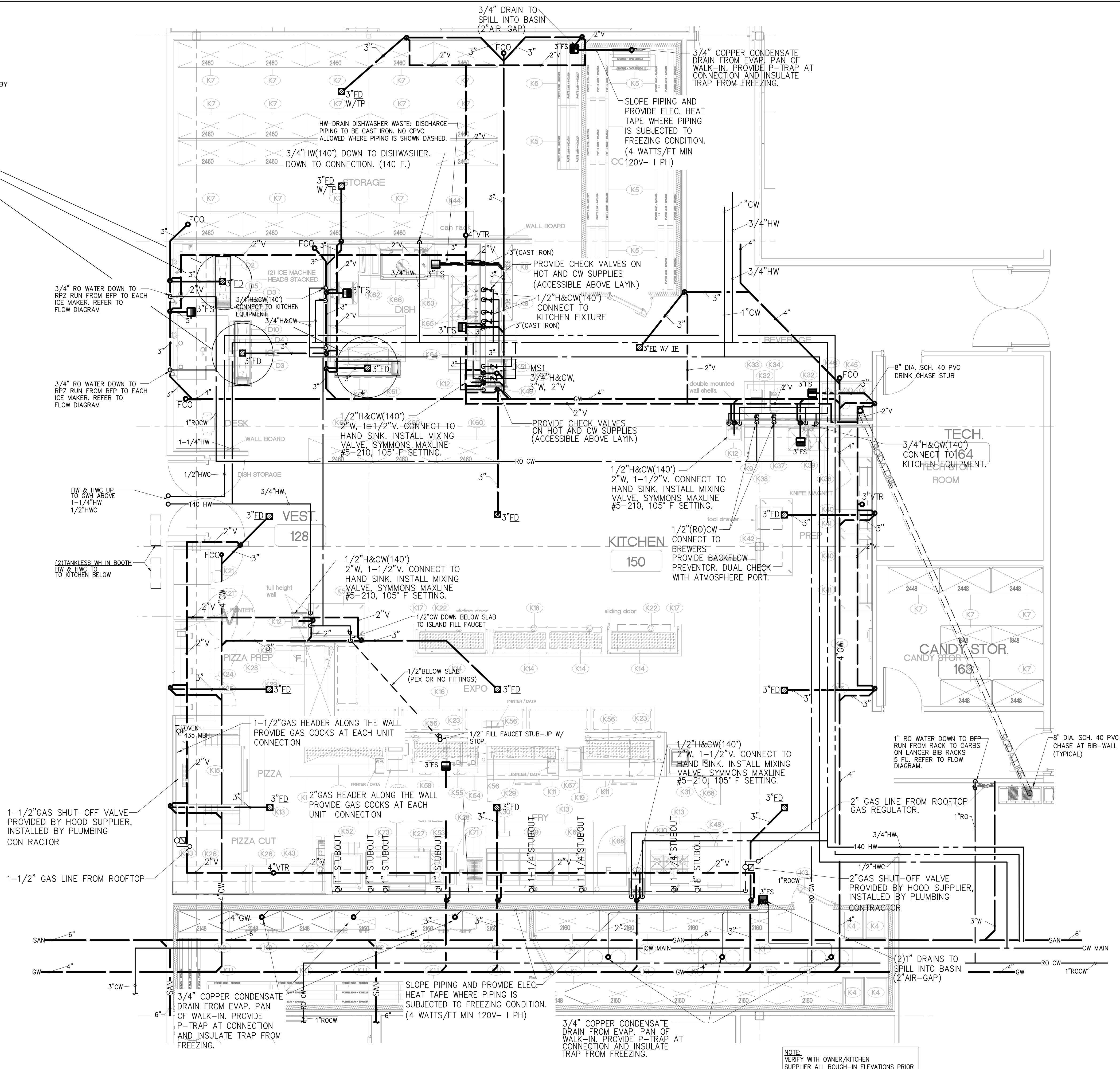
01 KITCHEN PLAN - PLUMBING Scale: 1/4"=1'-0"
