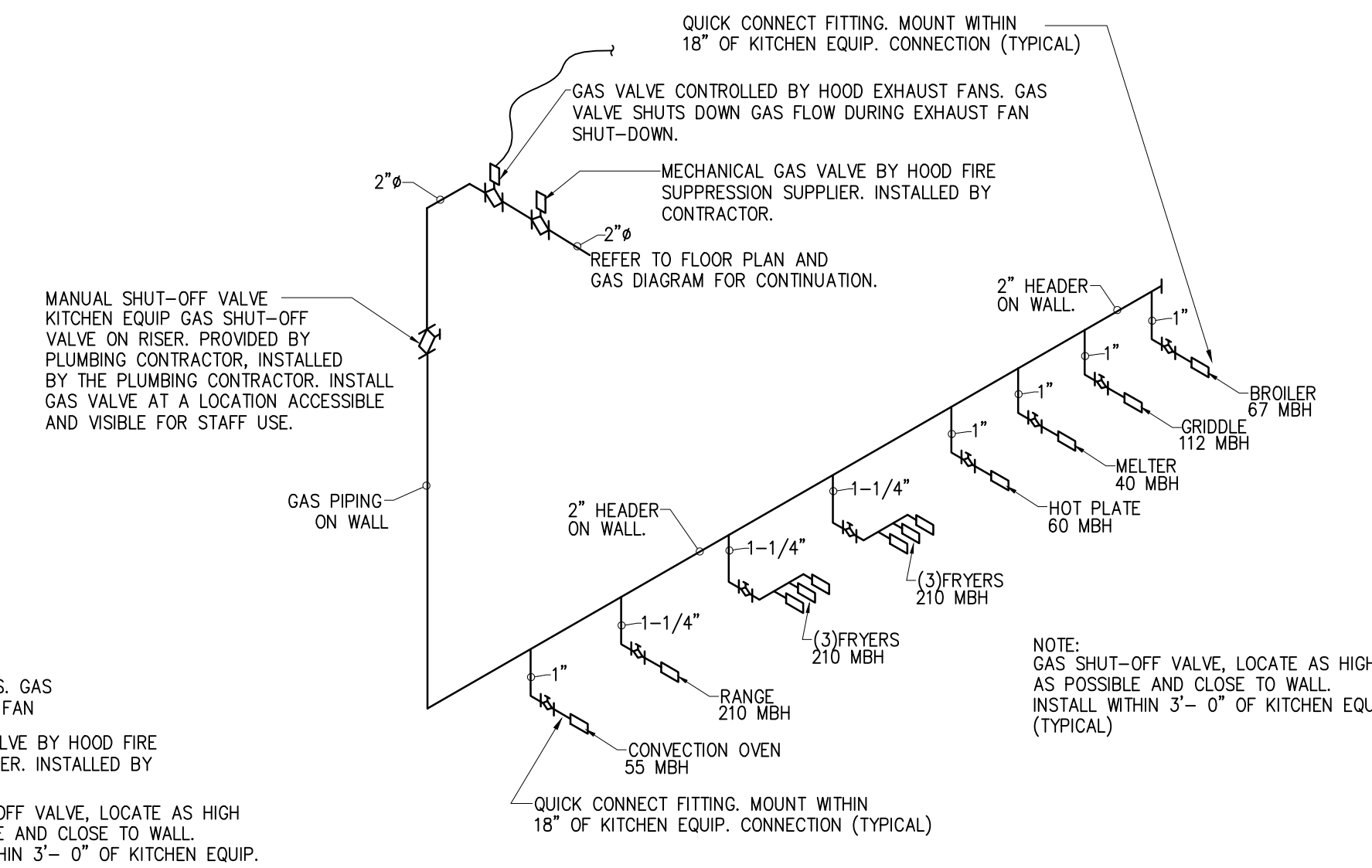
08 KITCHEN COOKLINE- GAS RISER Scale: NOT TO SCALE
