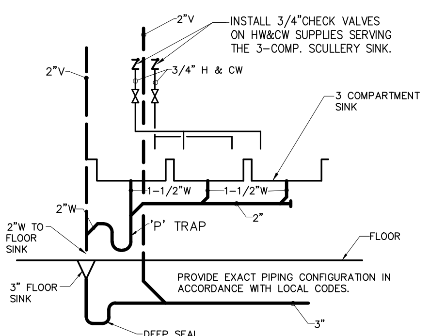
04 3-COMP. SINK DETAIL Scale: NOT TO SCALE
