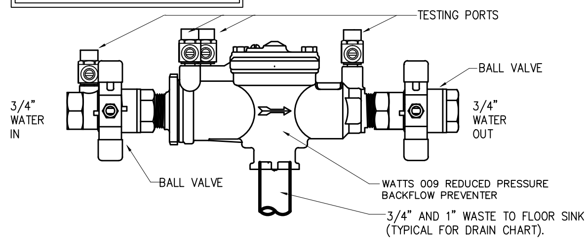
03 BACKFLOW PREVENTOR DETAIL Scale: NOT TO SCALE
