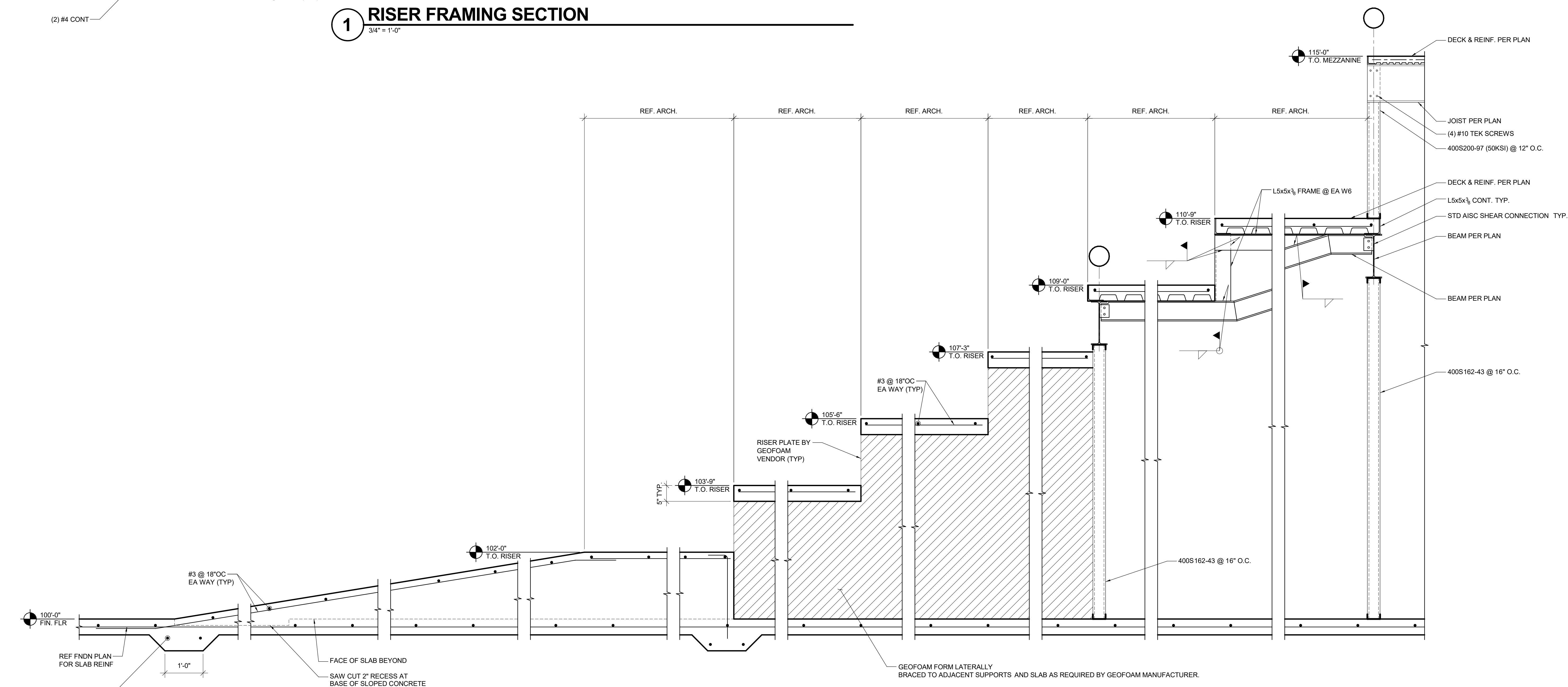
2 RISER FRAMING SECTION 3/4" = 1'-0"
