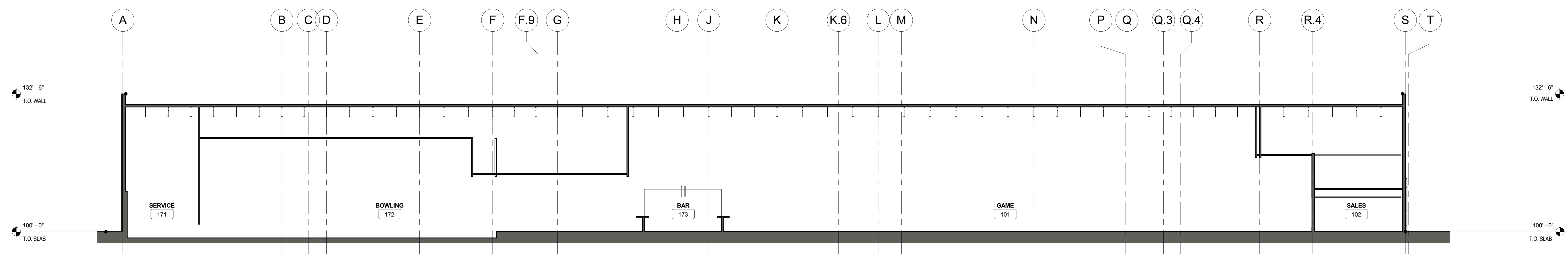
1 BUILDING SECTION AT GRID 6 TO GRID 7 3/32" = 1'-0"
