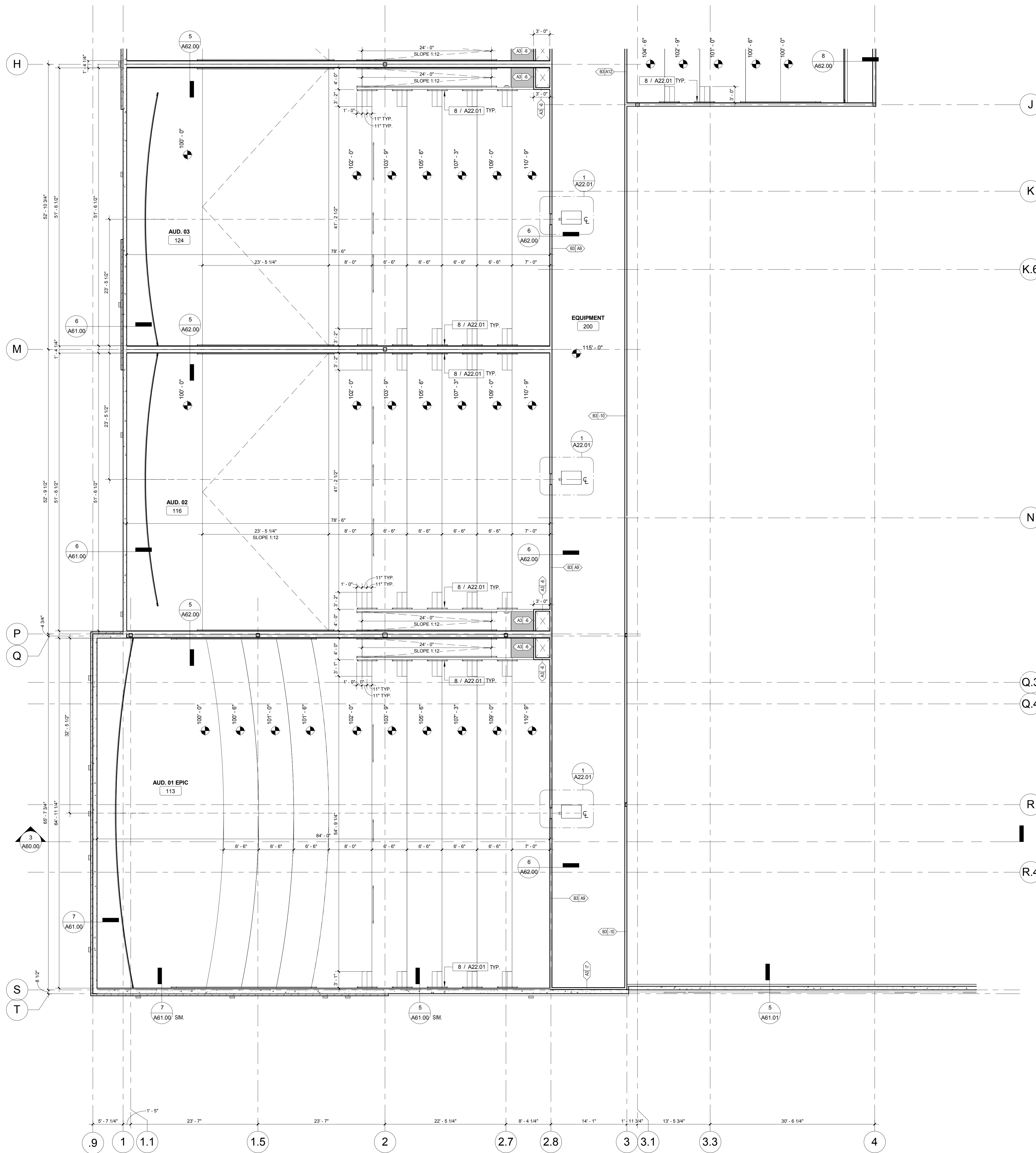
3 MEZZANINE FLOOR PLAN AREA 'C' 1/8" = 1'-0"
