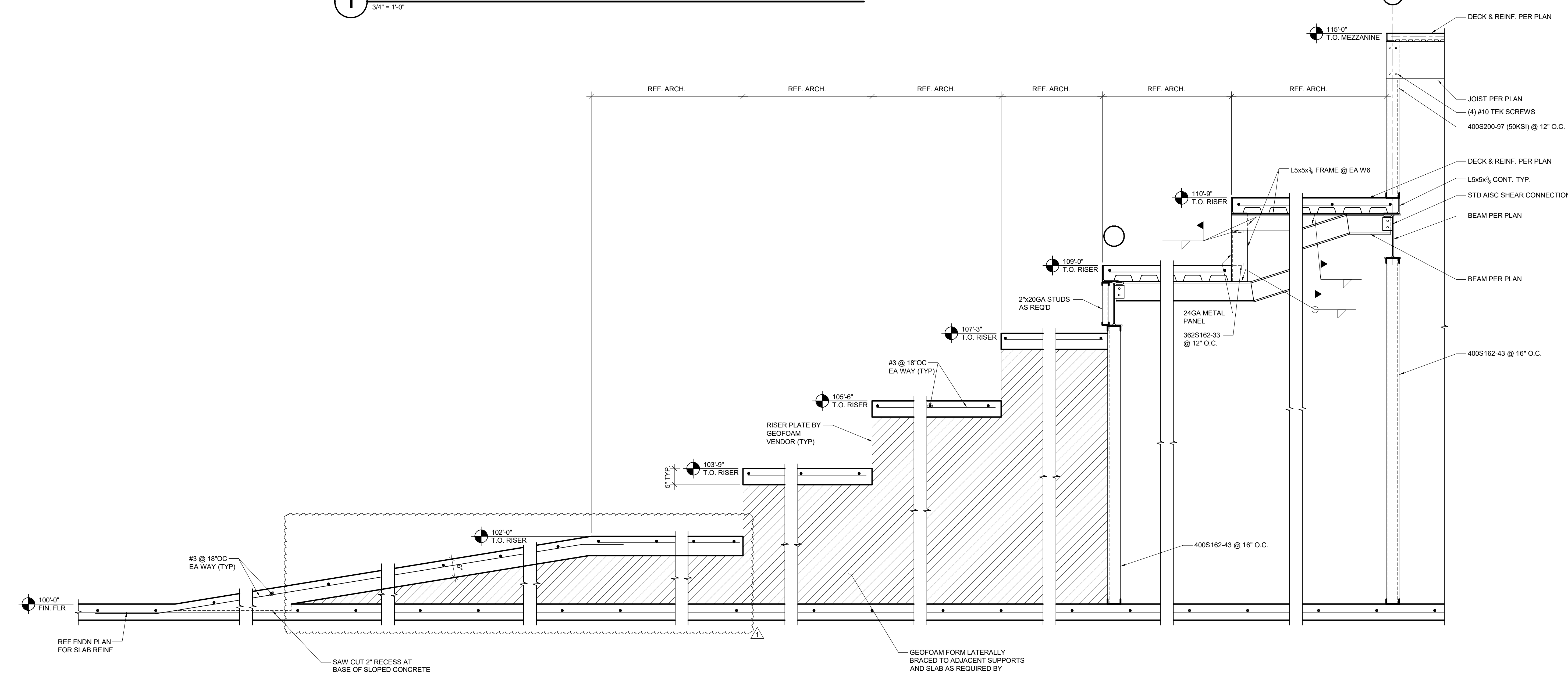
2 RISER FRAMING SECTION 3/4" = 1'-0"
