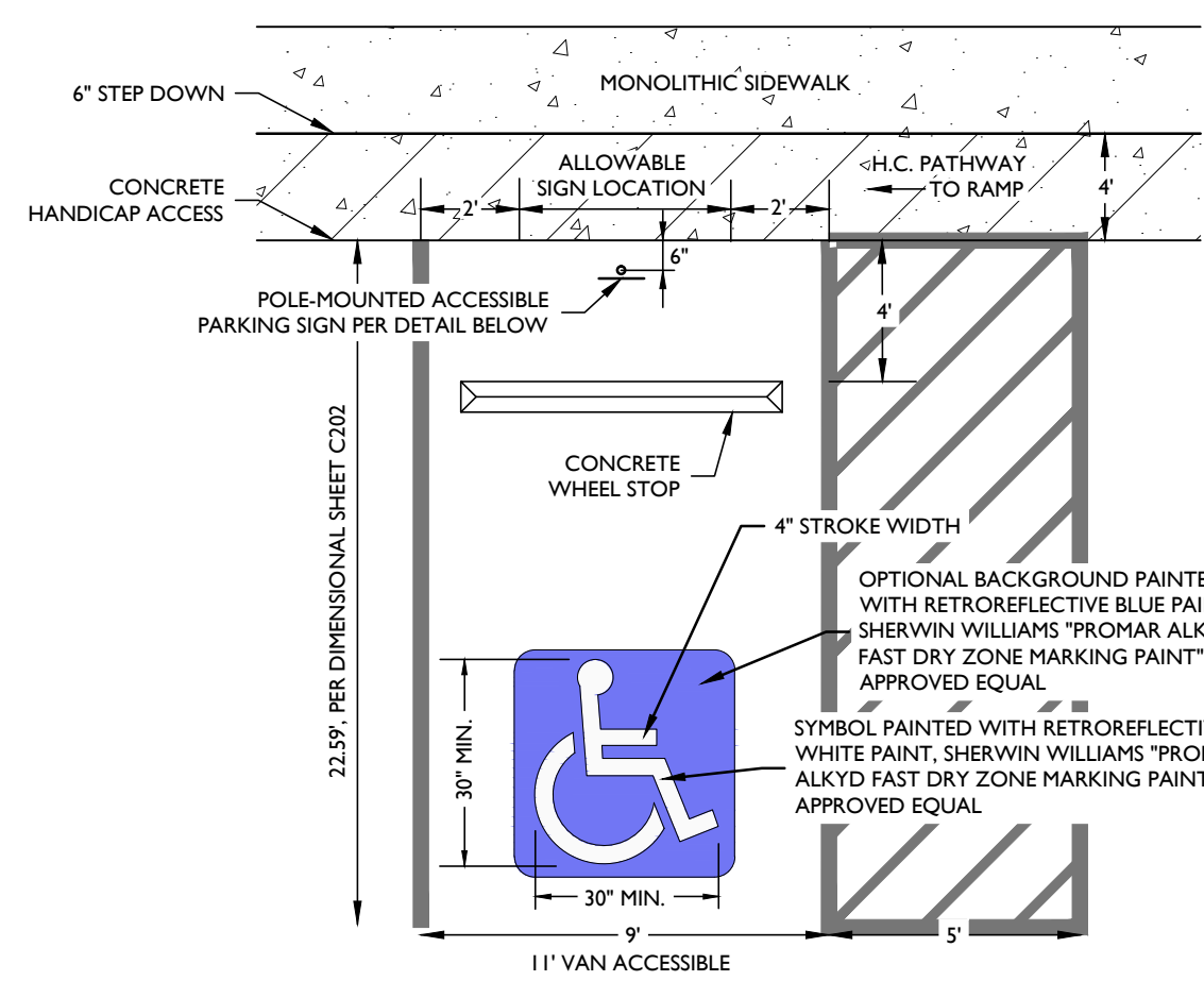
10 ACCESSIBLE SPACE MARKING "A" OR APPROVED EQUAL. N.T.S.
