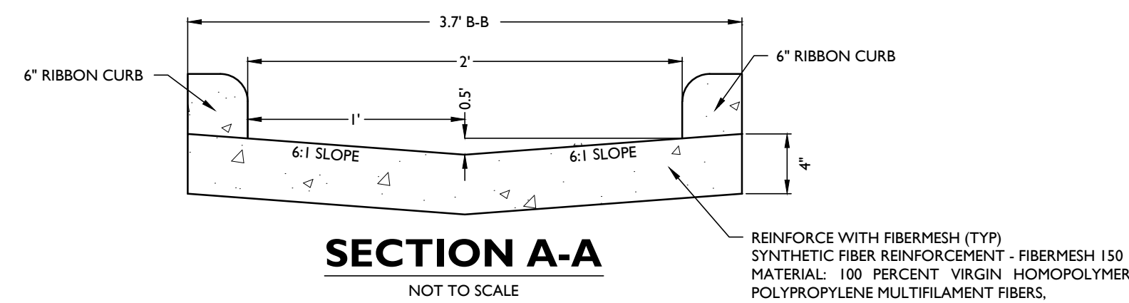
13 FLUME DETAIL OR APPROVED EQUAL. N.T.S.
