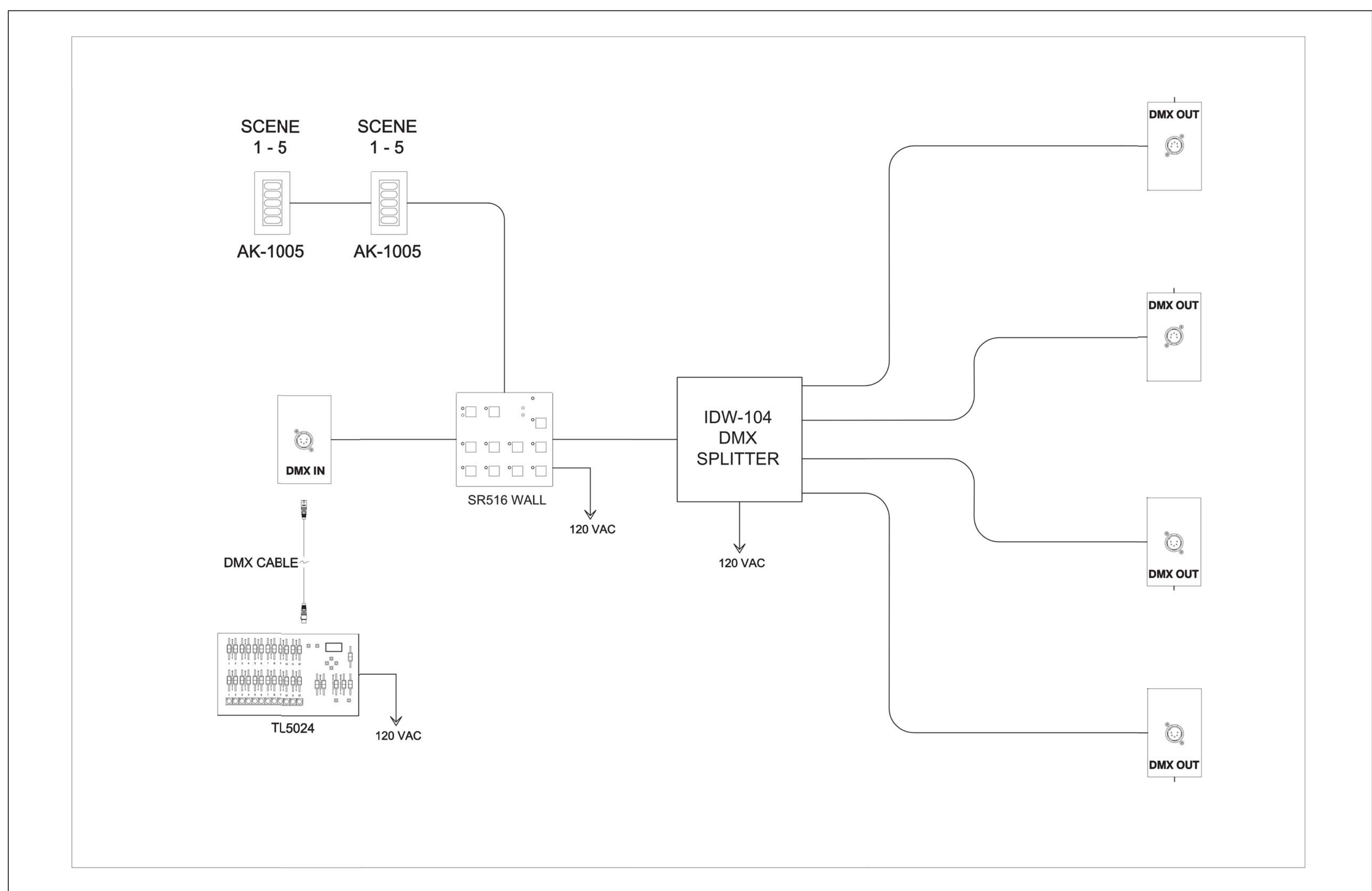
01 DMX INTERFACE WITH HOUSE LIGHTING AND AVL CONSOLE 1/4" = 1'-0"
