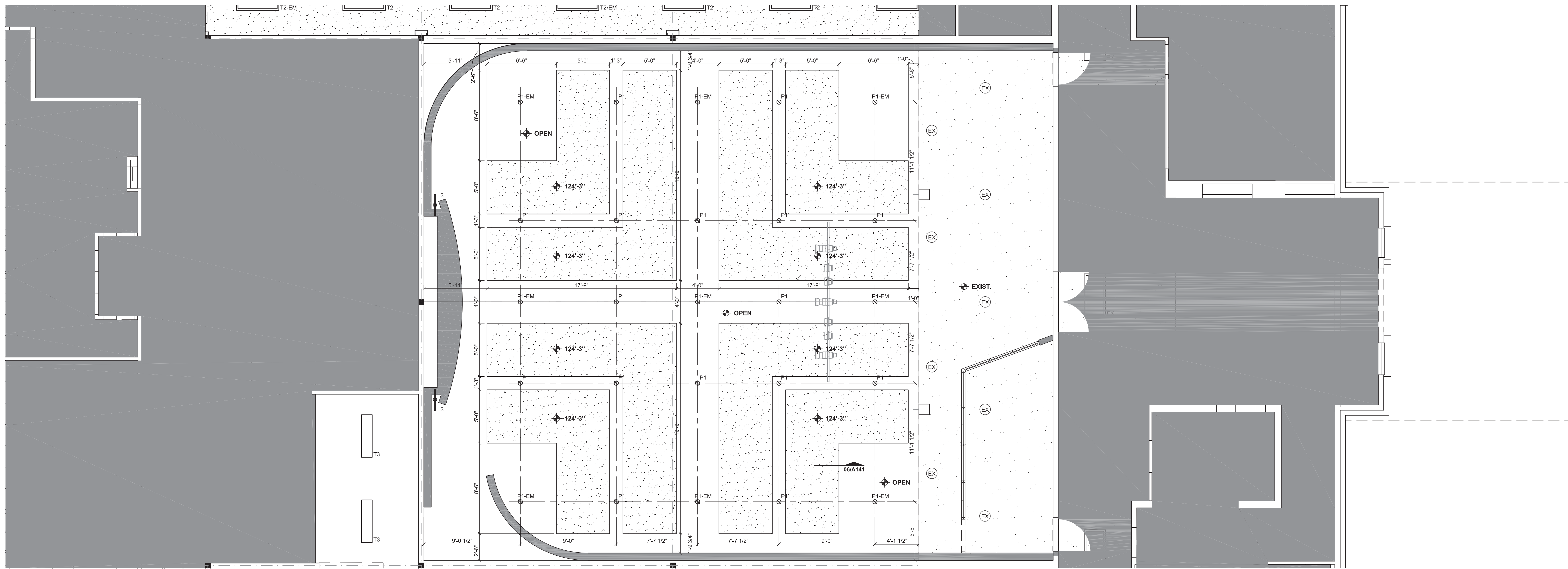
01 ENGLISH MINISTRY REFLECTED CEILING PLAN - LEVEL 1 1/4" = 1'-0"
