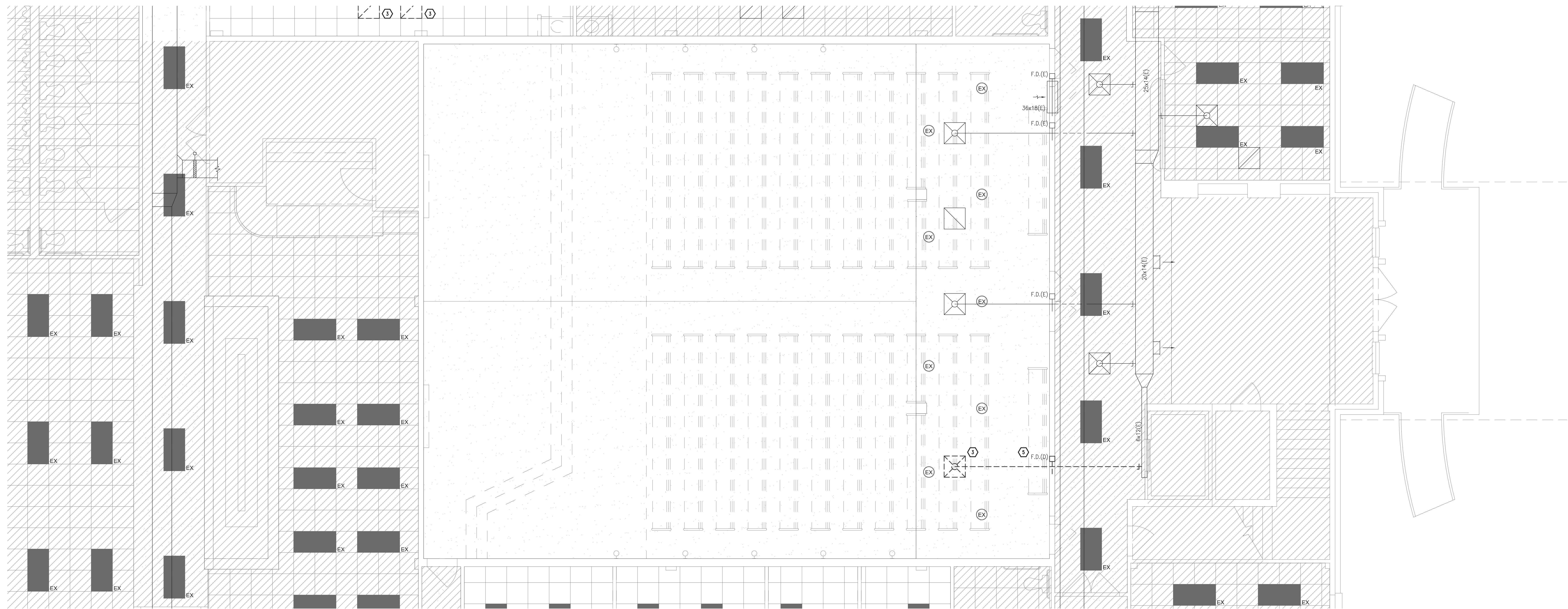
01 ENGLISH MINISTRY MECHANICAL DEMO FLOOR PLAN - LEVEL 1 1/4" = 1'-0"
