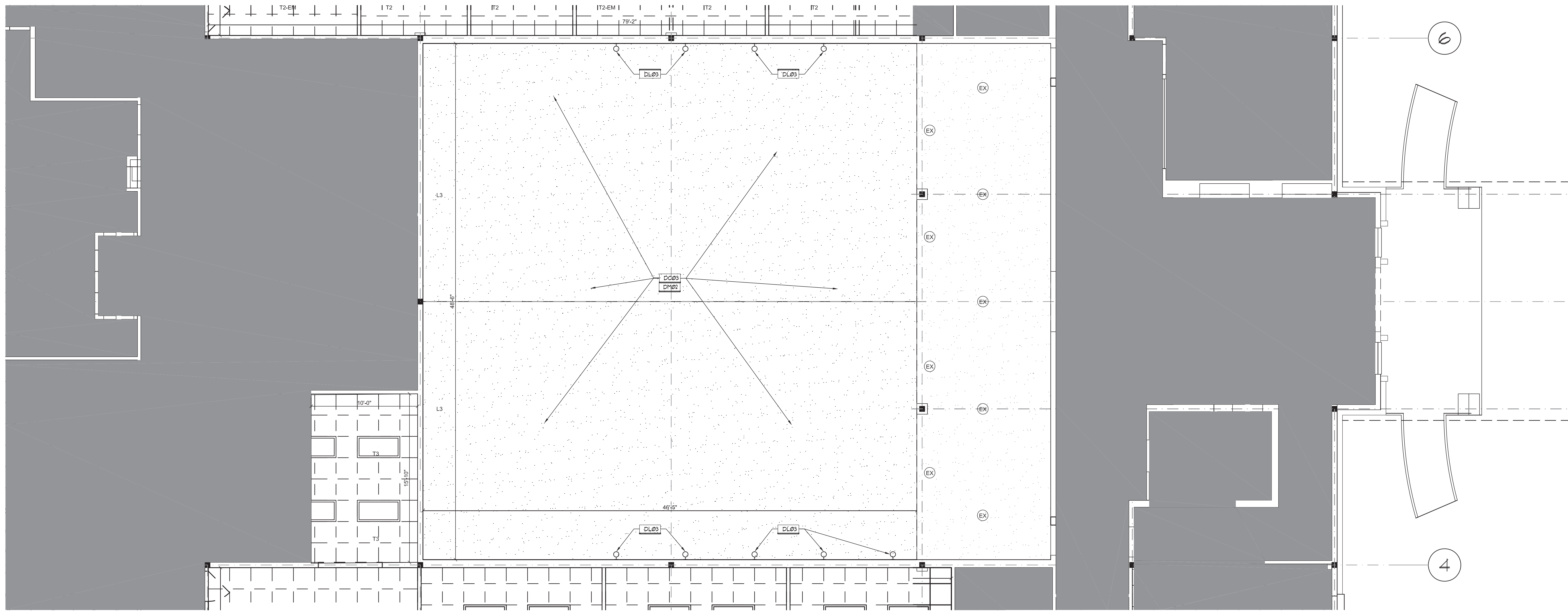
01 ENGLISH MINISTRY DEMOLITION REFLECTED CEILING PLAN - LEVEL 1 1/4" = 1'-0"
